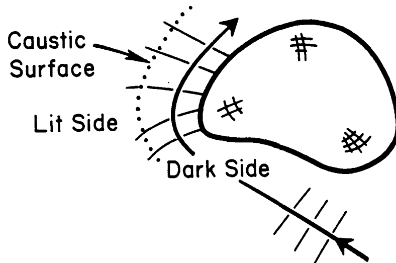
Figure 4. Heuristic Definition of Caustic
