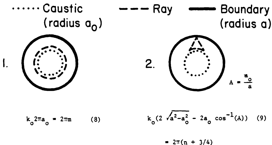
Figure 2. The Independent Paths
