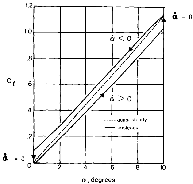
Figure 3. Hysteresis Effect Due to Unsteadiness
