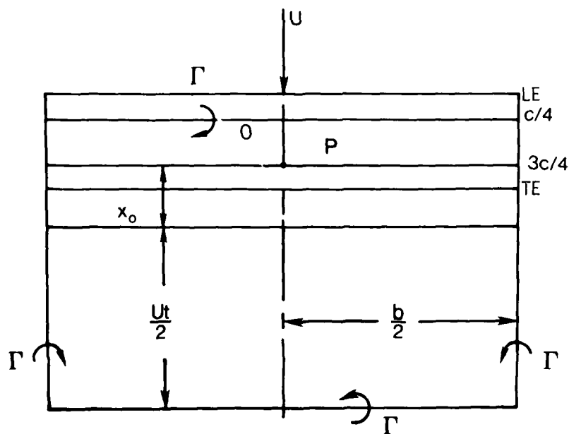
Figure 4. Simplified Vortex System for Straight Wings
