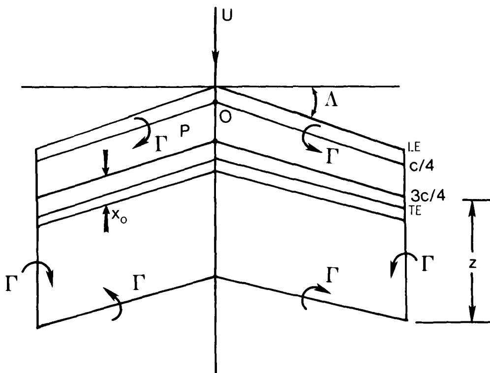
Figure 6. Simplified Vortex System for Swept Wings
