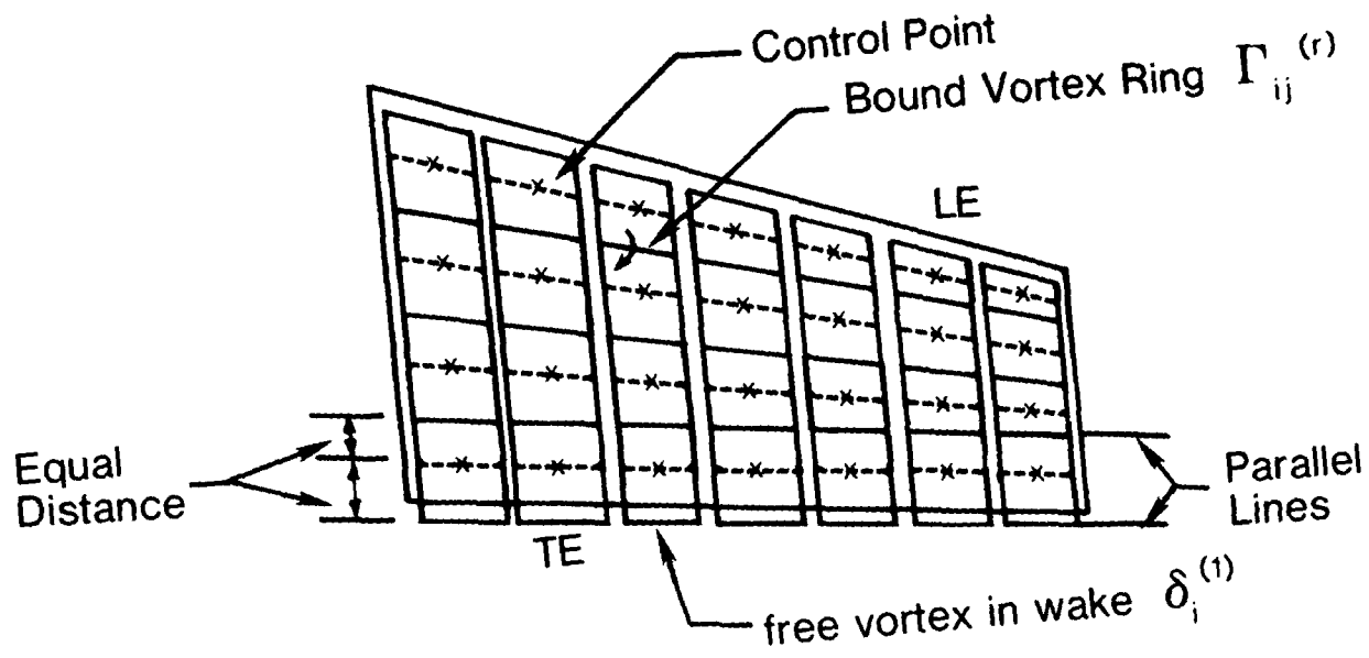
Figure 1. Vortex-lattice Method of Belotserkovskii
