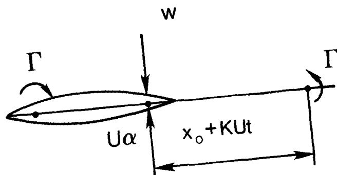
Figure 2. Simplified Vortex System
