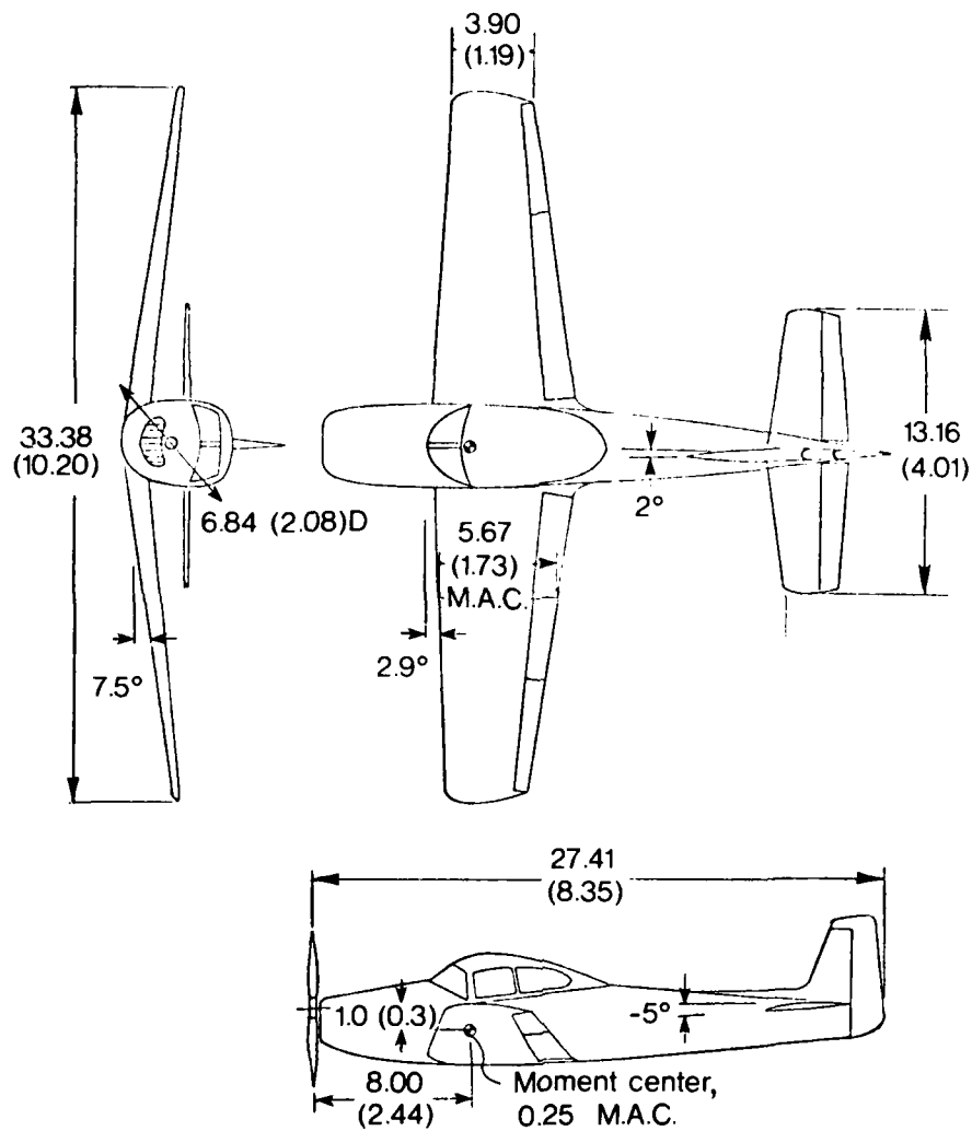
Figure 8. Sketch of Navion Aircraft
