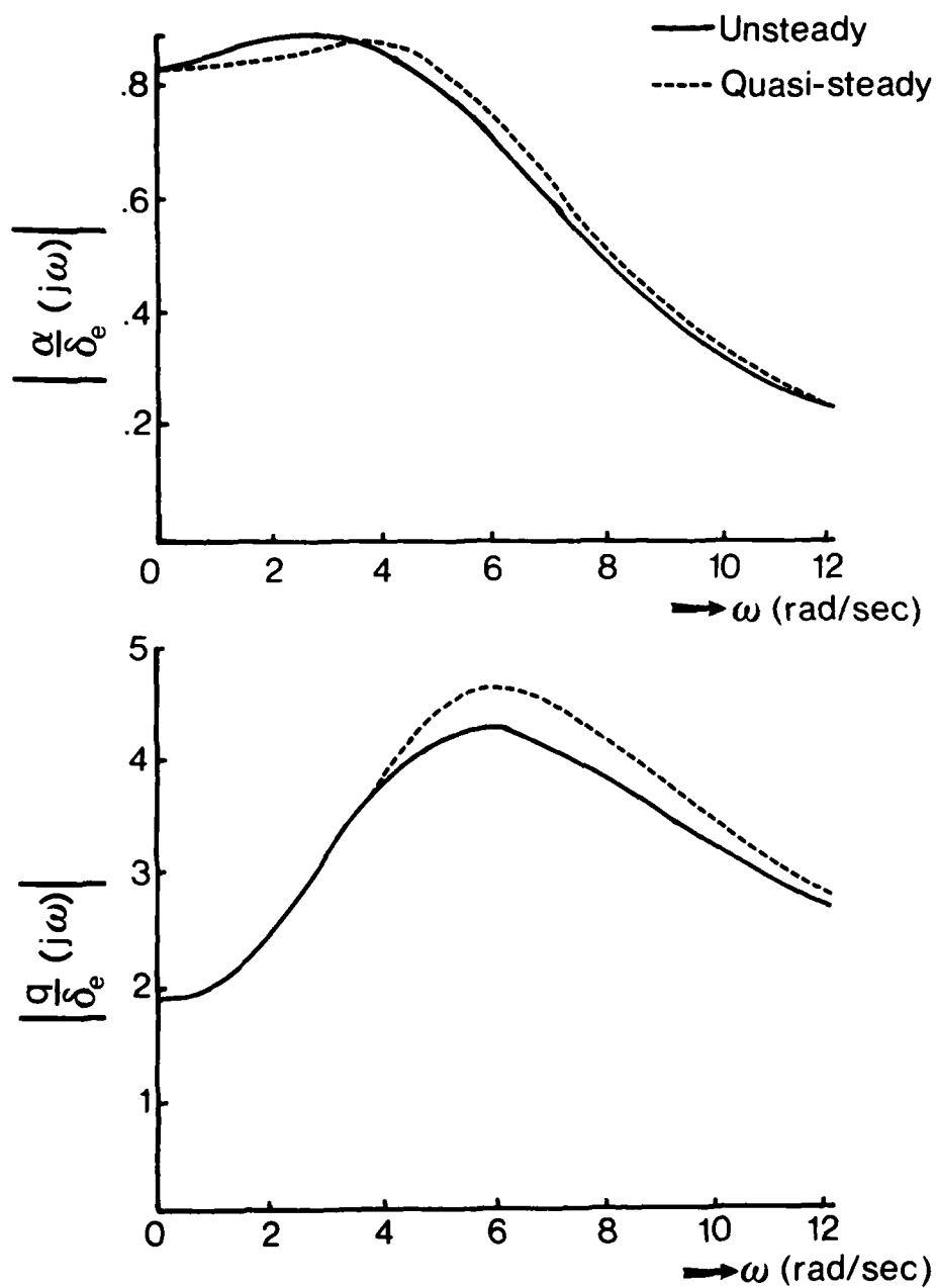
Figure 11. Frequency Response of Navion Aircraft
