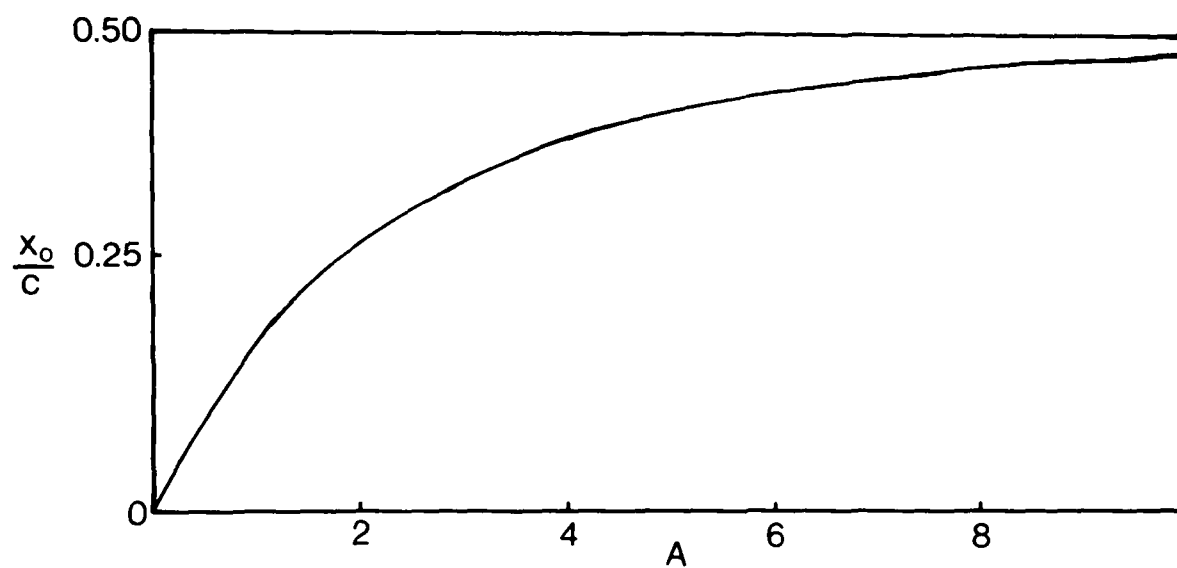
Figure 5. Variation of x_0/c With Aspect Ratio
