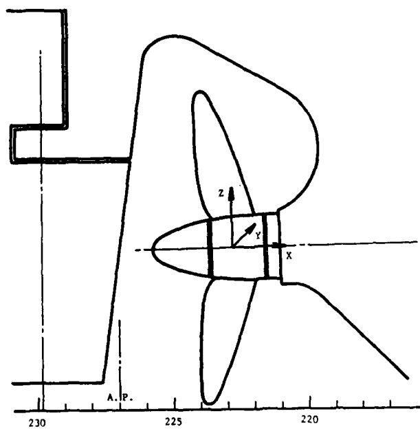
FIGURE 34. PROPELLER IN APERTURE
