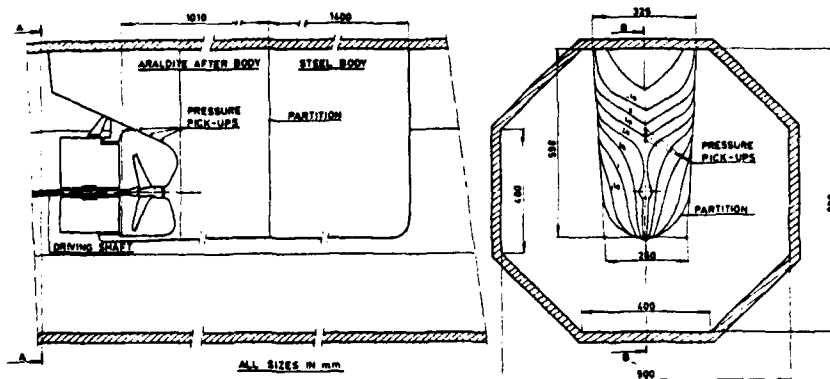
FIGURE 5. STERN GEOMETRY FOR CAVITATION TUNNEL TESTS, FROM [48]
