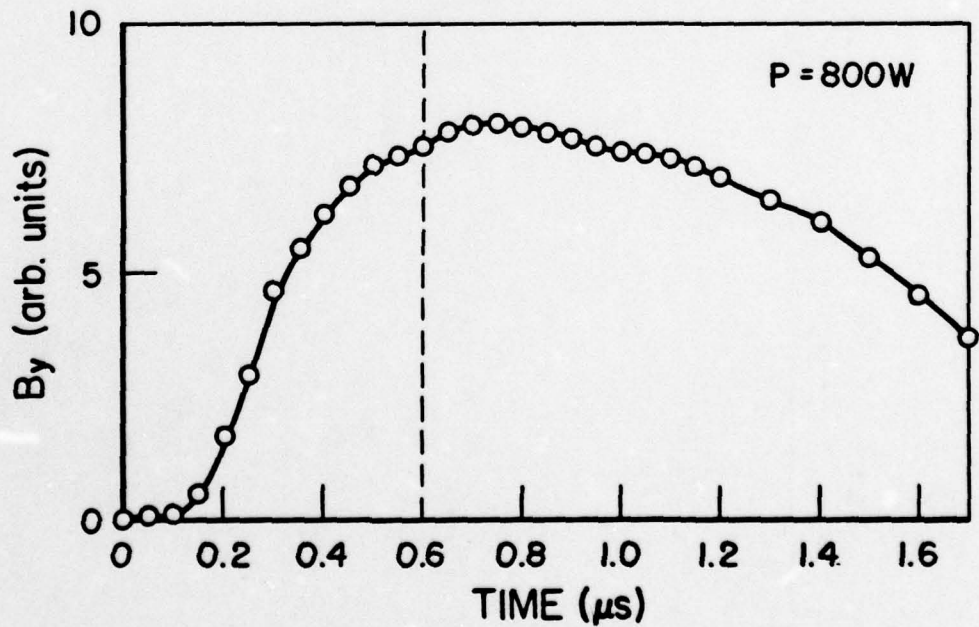
Fig. 9. Coincidence of Saturation Times for Electric and Magnetic Fields.
