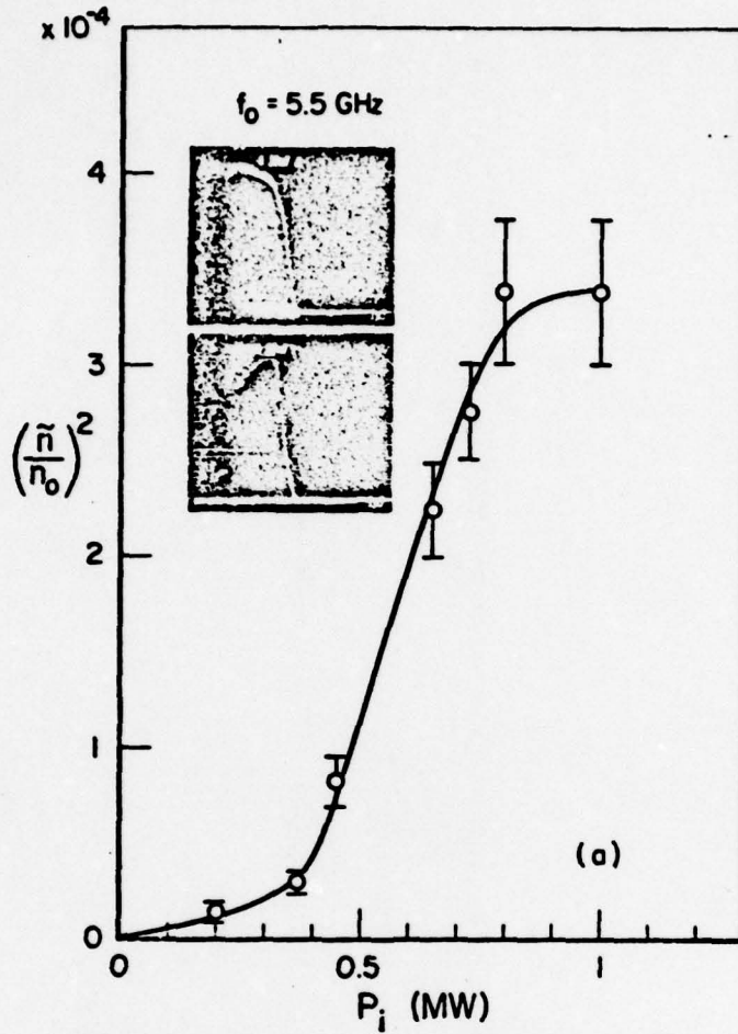
Ion wave amplitude ( Z = 60\text{cm} ) versus incident power ( \tau_p = 4 \mu\text{sec} )
