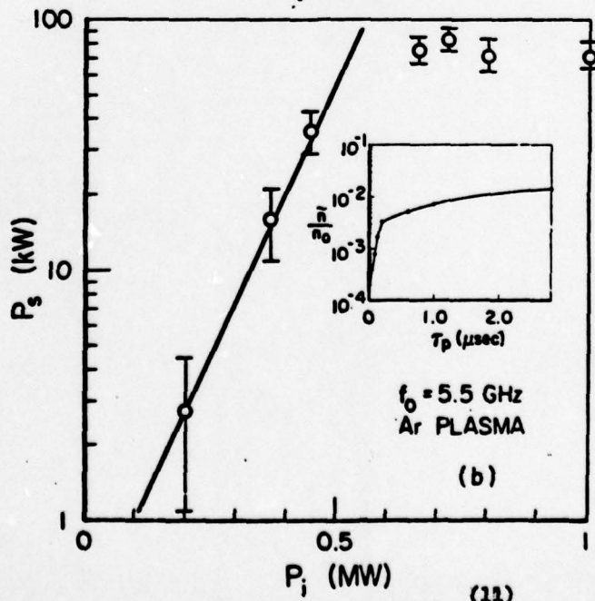
Scattered power versus incident power ( \tau_p = 4 \mu\text{sec} )
