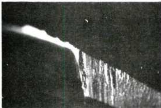
Fig. 66: Grooved Wear on the Margin
