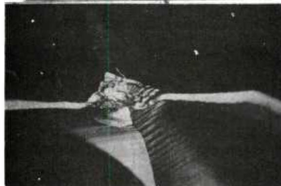
Fig. 78: Wear on Drills a) Helical b) Racon
