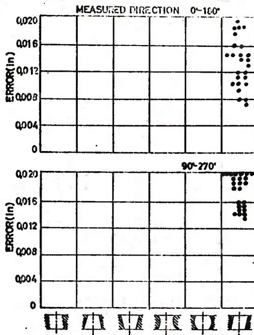
Fig. 46: The Straightness Errors Produced by the Sloped Workpiece Surface to the Axis of the Spindle
