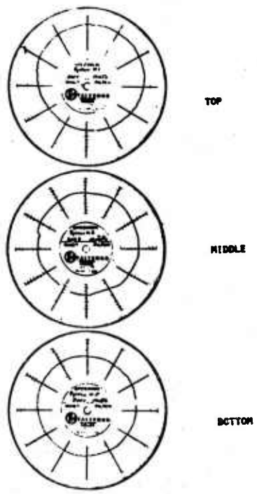
Fig. 82: Roundness Measuring Record of the Hole Drilled a) Helical Point Drill c) Roundness Measuring Record of b) Racon Point Drill the Hole Drilled - Pyrcan Drill
