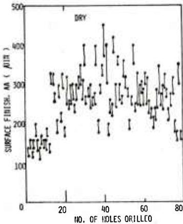
Fig. 60: Surface Finish Using Cutting Fluid (a) and Dry Condition (b)
