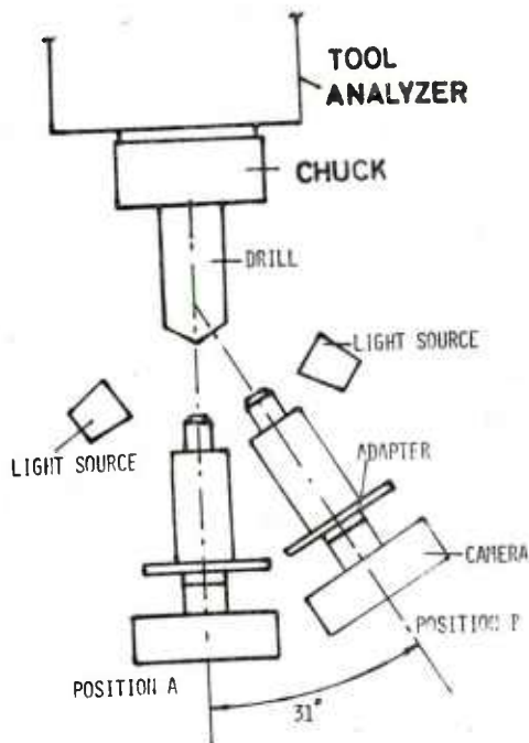
Fig. 17: Device for Photography of Progress of Wear
