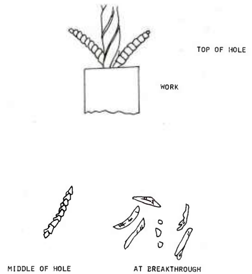
Fig. 52: Chips Being Emitted in Drilling and Different Types of Chip (Schematic)
