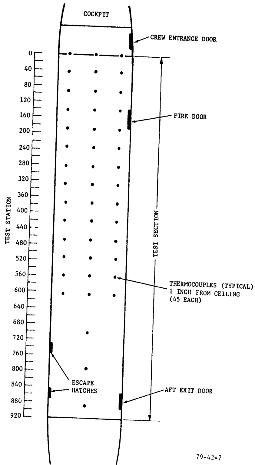
FIGURE 7. TEST ARTICLE CEILING THERMOCOUPLE LOCATIONS
