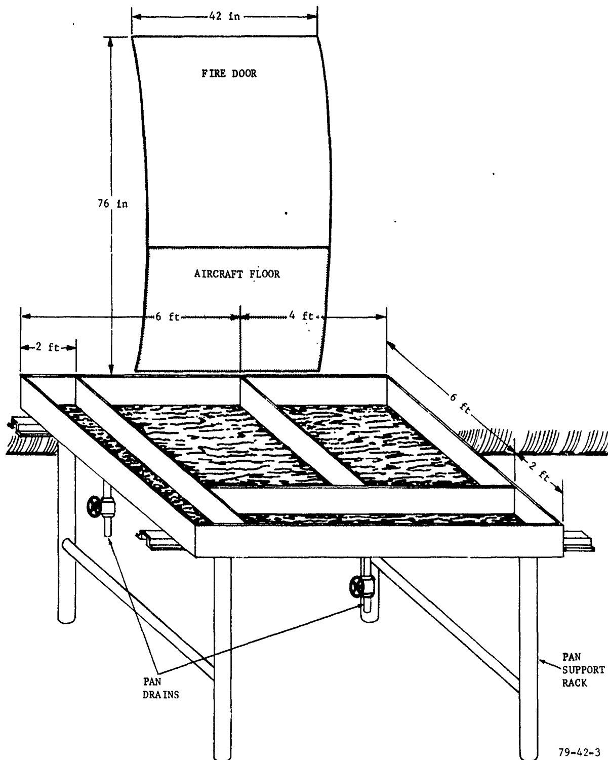
FIGURE 3. FIRE PAN INSTALLATION
