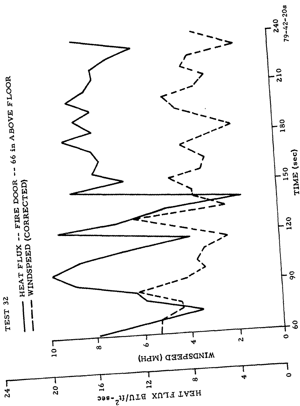
FIGURE 20. EFFECT OF WIND VARIATION ON WIND ENTERING FUSELAGE (Sheet 1 of 2)
