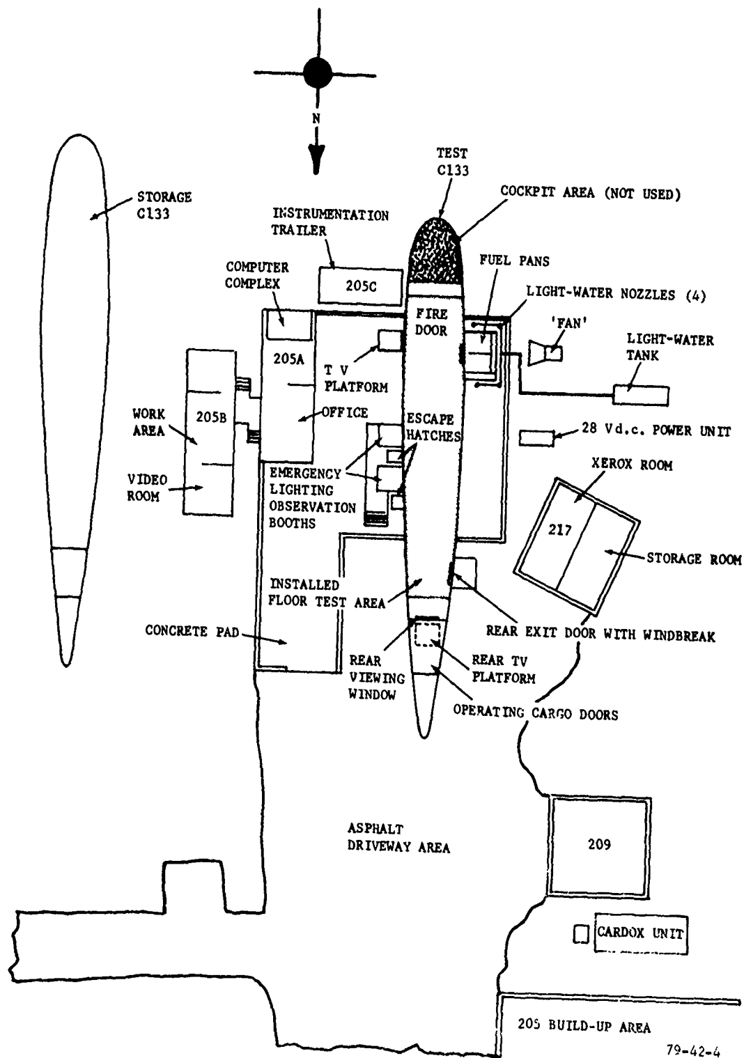
FIGURE 4. FULL-SCALE FIRE TEST FACILITY
