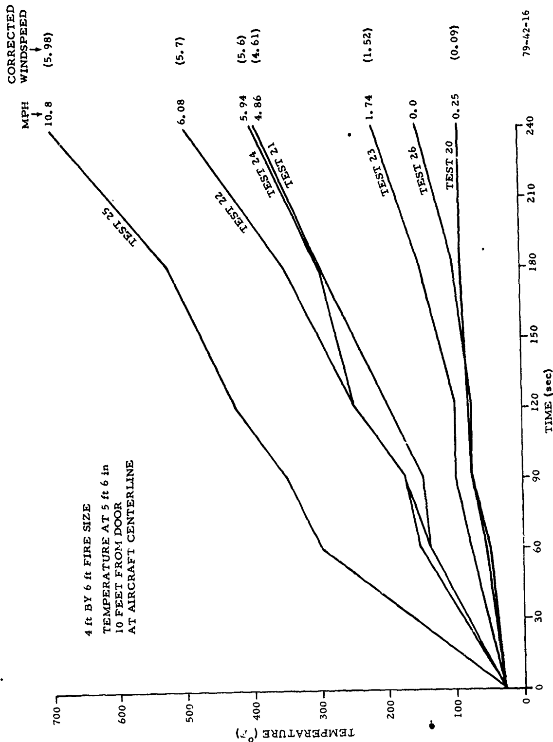
FIGURE 16. EFFECT OF WIND ON CABIN TEMPERATURES (4- BY 6-FOOT FIRE)
