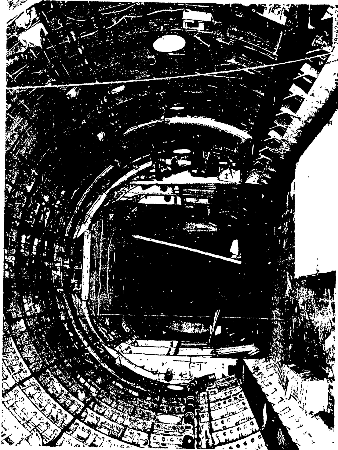
FIGURE C-2. FUSELAGE INTERIOR, PRIOR TO INSTALLATION OF TEST SECTION FLOOR, FIRE RESISTANT SIDEWALL COVERINGS AND CEILING
