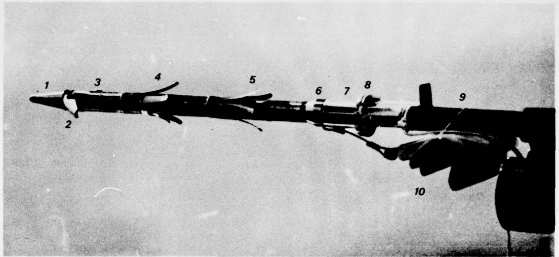
Figure 5. Radio whale tag used on B. edeni , off Venezuela, October and November 1979. The tag is made of stainless steel. Components of the tag, starting from the left: (1) point, (2) folding toggles, (3) pressure case with two sets of "hula skirt" (4 and 5) projections, (6) antenna flange, (7) release couplings, (8) pushrod flange, (9) barrel of shoulder-gun, and (10) folded plastic streamer. The new modifications for these experiments were the hula skirt projections (4 and 5) for increased holding area in the blubber, and flange and release couplings (6 and 7) which reduces external drag and sets the tag antenna below the skin. (Photo by Watkins)
