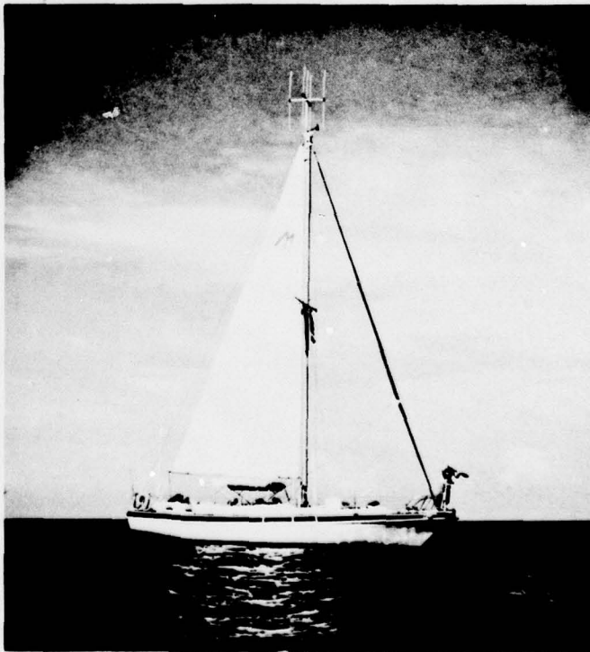
Figure 6. Tagging and tracking arrangements on a Morgan 41 sloop. A platform was constructed on the bow ahead of the mast stay for unobstructed tagging, and the Adcock ADF antennas were mounted at the top of the mast. (Photo by Moore)
