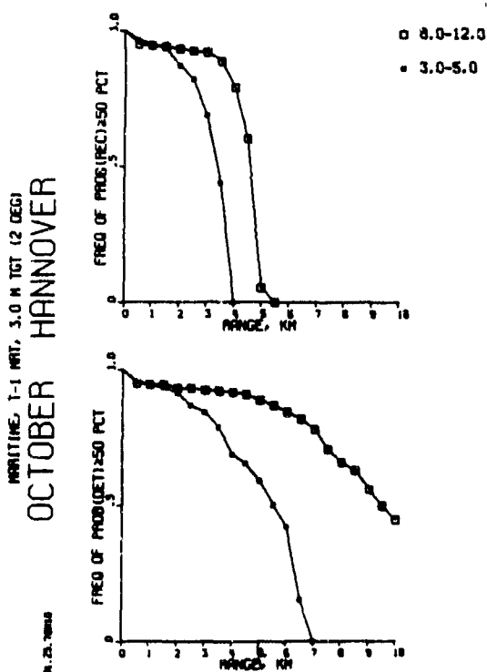
FIGURE 3. Seasonal probabilities of detection and recognition of tank in front aspect by 3-5 and 8-12 \mu m FLIRs, assuming maritime aerosol model.
