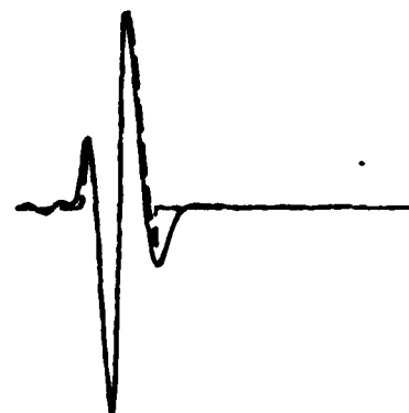
Figure 21. An inversion test introducing arbitrary "noise" to the synthetic data. The dashed seismogram is the same as in Figure 20 except that the fourth peak amplitude is reduced to 1/2 its previous value. The initial source parameters used in (a) are the same parameters used for the synthetic data. The inversion program is then allowed to go through four iterations under two different circumstances: (b) shows the results when using peak amplitudes and peak times as data, and (c) shows the results when using only the peak amplitudes as data.
