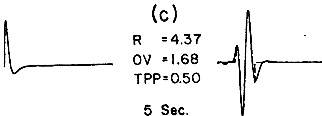
Figure 20. An inversion test to retrieve the source parameters of synthetic data. The dashed seismogram in (a), (b), and (c) is constructed from a synthetic using t^* = 1.0 , R = 5.0 , OV = 2.0 , TPP = 0.50 . The initial input trial source and the resultant synthetic are shown in (a), with (b) and (c) showing the results of the first two iterations respectively. As can be seen there is an excellent visual correspondence after just two iterations.
