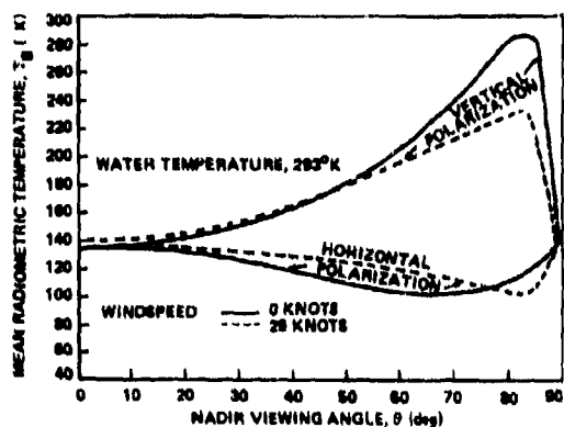
Figure VI-4. Theoretical antenna temperatures for sea state as functions of nadir viewing angles and wind velocity.
