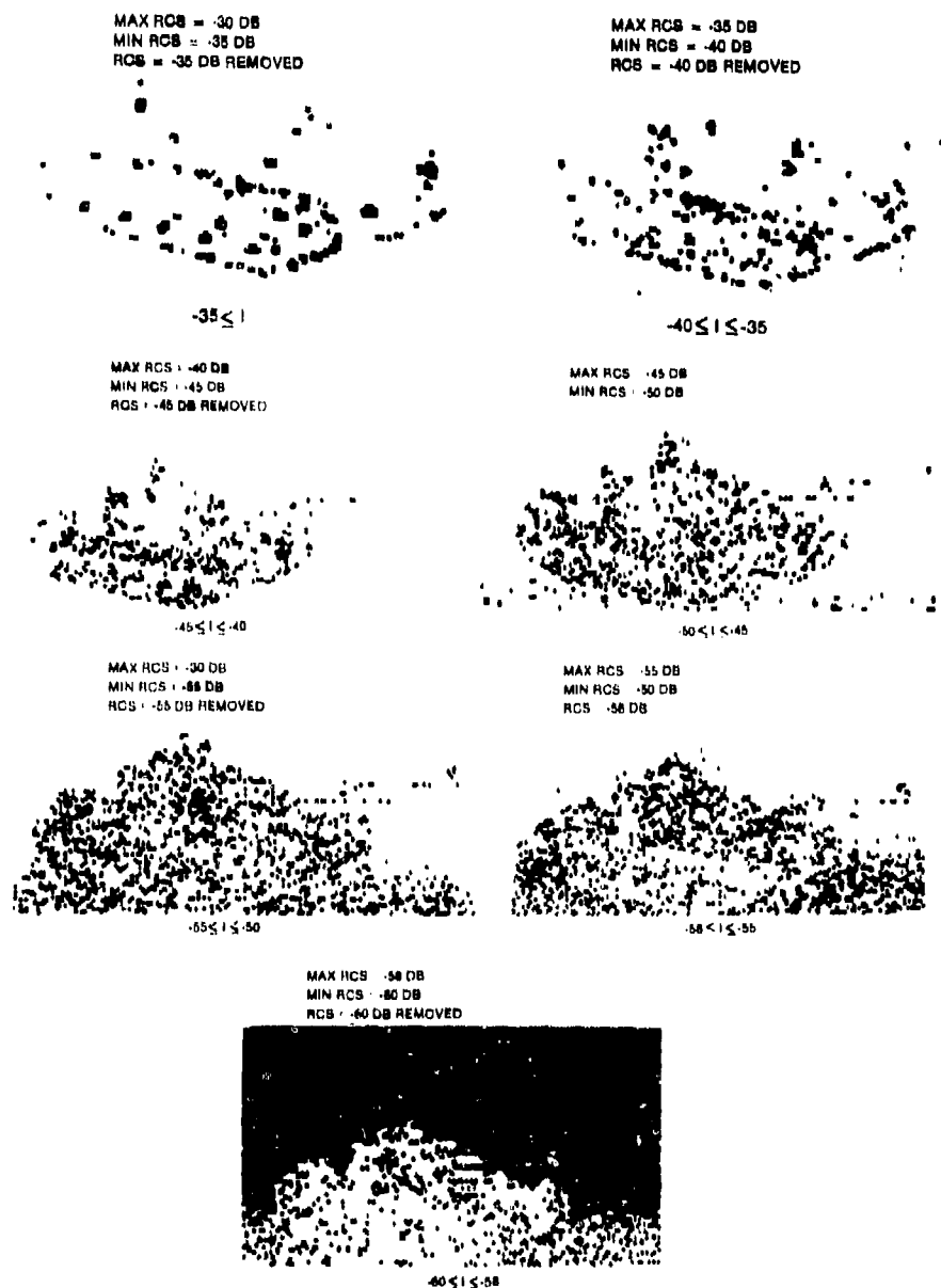
Figure VI-3(b). Level-sliced images of M48 tank and surrounding terrain (level-slicing intervals in dB), HV polarization.
