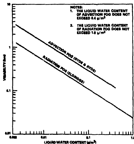
Figure III-6. Correlation of visibility in fog with liquid water content. R. G. Eldridge, Journal of Atmospheric Science , vol. 123 (1966).
