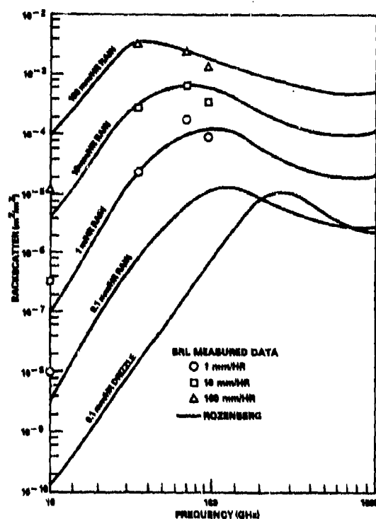
Figure III-17. Calculated and measured rain backscatter coefficient versus frequency. V. W. Richard, Ballistic Research Laboratories, Memorandum Report 2631 (June 1976).
