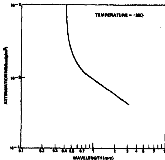
Figure III-21. Plot of ice cloud or ice fog attenuation versus wavelength.
