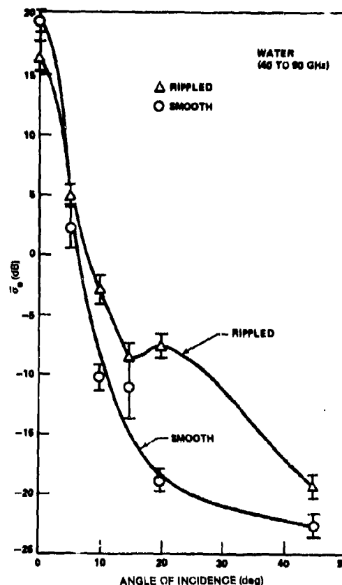
Figure VI-7. Mean \sigma_0 for smooth and rippled water, 40 to 90 GHz.
