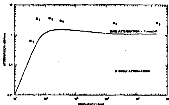
Figure I-25. Measured snow attenuations as a function of frequency. Snowfall rate of 1 mm (liquid)/hr. (1) Robinson (1955), (2) Lammers (1967), (3) BRL, (4) Babkin et al (1970), and (5) Sokolov (1970). Comparison curve shown for equivalent rainfall.
