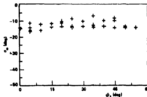
Figure VI-25. \sigma_0 versus \phi_s for HH polarization, \theta_i \sim 79 deg and \theta_s = 85 deg, \lambda = 3 cm (grass and cement ramp).
