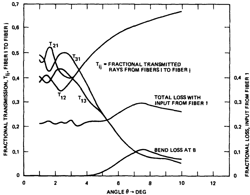
(c) TRANSMISSIONS AND LOSSES OF CONFIGURATION (b)
