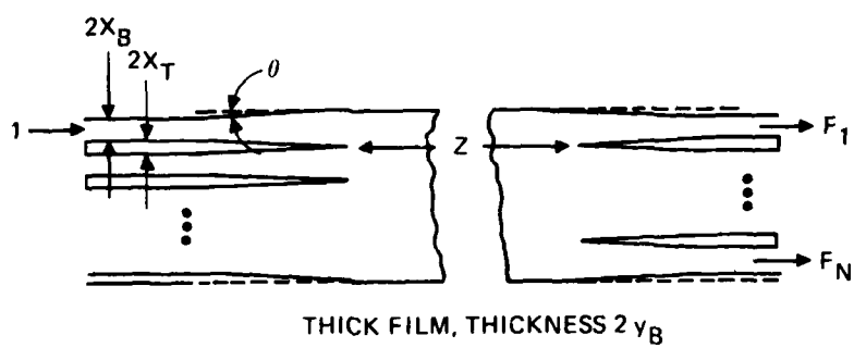
Figure 2. Schematic of a planar star coupler.
