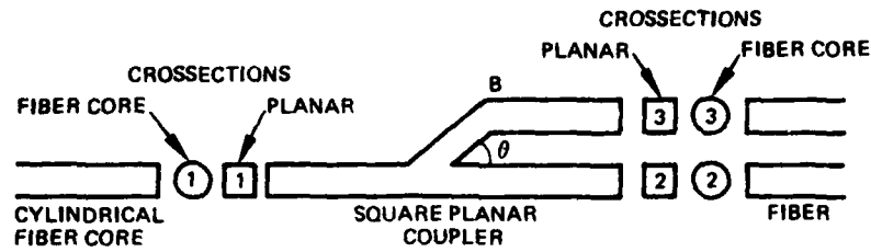
(b) FIBER TO PLANAR Y W/BEND TO FIBER
