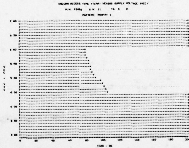
FIGURE F23. 93481 SHMOOS FOR COLUMN ADDRESS ACCESS TIME - ROWPAT PATTERN
