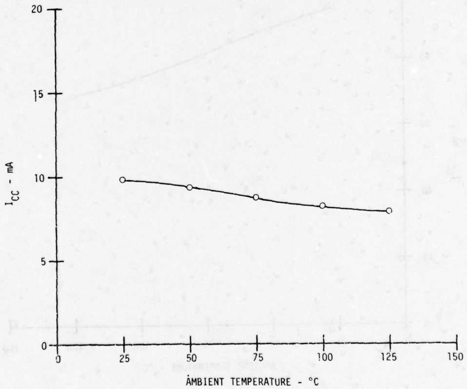
FIGURE 7-4. FAIRCHILD 93481 STATIC BURN-IN CIRCUIT EVALUATION
