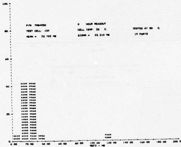
FIGURE F4. TMS4050 HISTOGRAMS OF REFRESH TIME - CHECKERBOARD PATTERN
