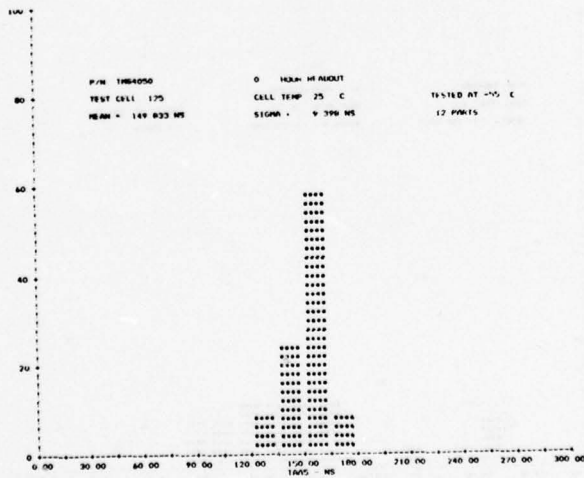
FIGURE F3. TMS4050 HISTOGRAMS OF ADDRESS ACCESS TIME - MARCHING PATTERN
