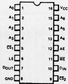
FIGURE D1. TERMINAL CONNECTION
