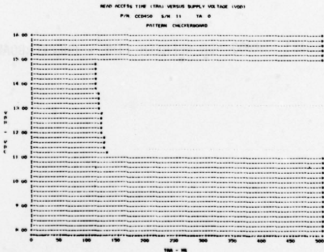
FIGURE F25. CCD450 SHMOOS FOR READ ACCESS TIME - CHECKERBOARD PATTERN
