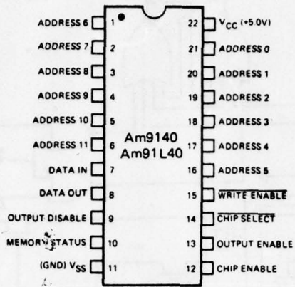
FIGURE B1. TERMINAL CONNECTION
