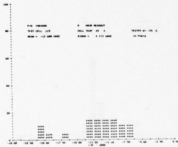
FIGURE F2. TMS4050 HISTOGRAMS OF SUPPLY CURRENT FROM V_{BB} SUPPLY
