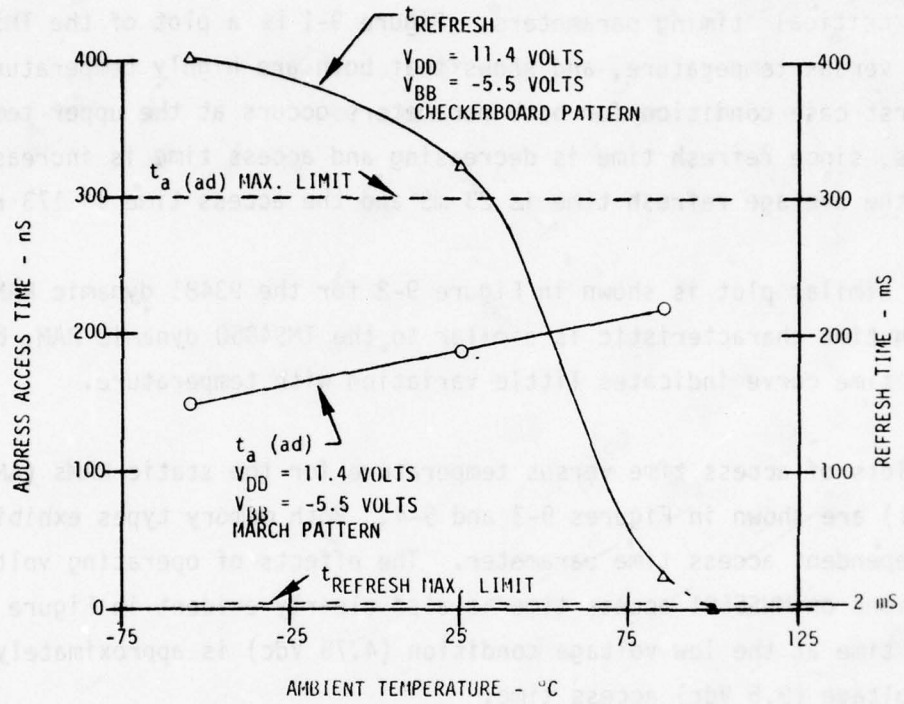
FIGURE 9-1. TEXAS INSTRUMENTS TMS4050 AVERAGE ADDRESS ACCESS TIME AND AVERAGE REFRESH TIME VERSUS AMBIENT TEMPERATURE
