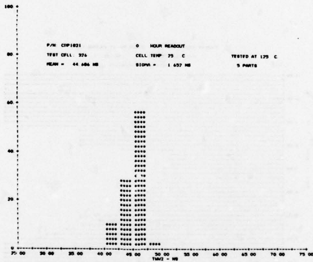
FIGURE F18. CDP1821 HISTOGRAMS OF ADDRESS ACCESS TIME - WALKING PATTERN
