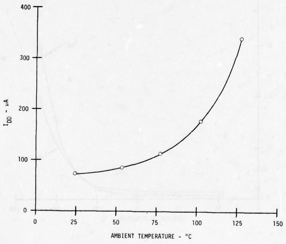
FIGURE 7-1. RCA MWS5501 STATIC BURN-IN CIRCUIT EVALUATION
