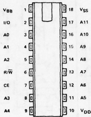
FIGURE A1. TERMINAL CONNECTION
