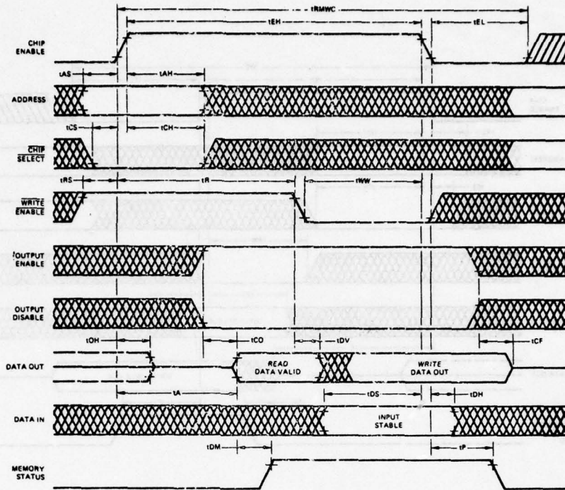
a) TIMING DIAGRAM
