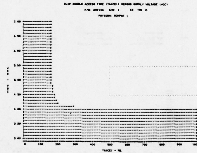
FIGURE F8. AM9140 SHMOOS FOR CHIP ENABLE ACCESS TIME - ROWPAT PATTERN
