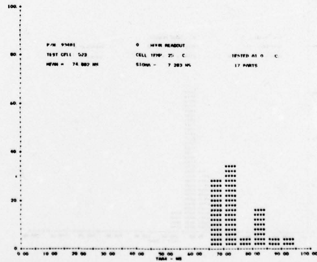
FIGURE F21. 93481 HISTOGRAMS OF COLUMN ADDRESS ACCESS TIME - ROWPAT PATTERN
