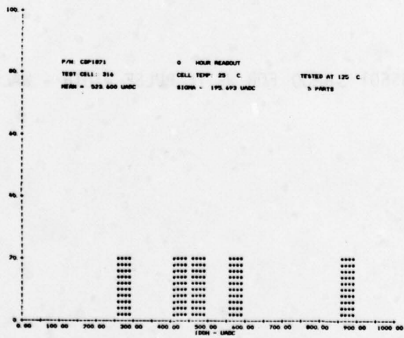
FIGURE F15. CDP1821 HISTOGRAMS OF SUPPLY CURRENT WITH V_{DD} = 10.5 VOLTS
