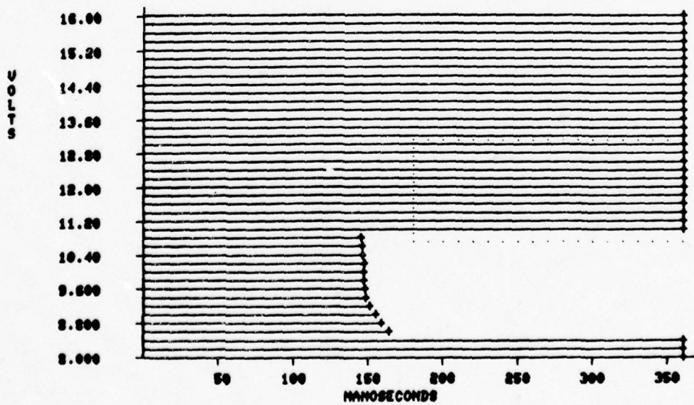
FIGURE 5-8. FAIRCHILD CCD450 ACCESS TIME SHMOOS SHOWING PATTERN SENSITIVITY AT HIGH TEMPERATURE
