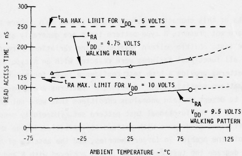
FIGURE 9-4. RCA MWS5501 AVERAGE READ ACCESS TIME VERSUS AMBIENT TEMPERATURE
