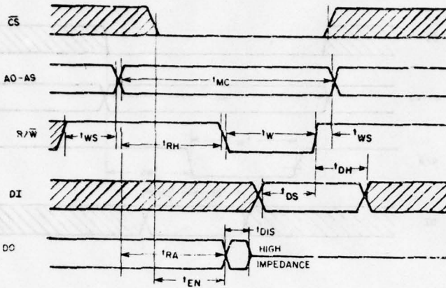
a) TIMING DIAGRAM
