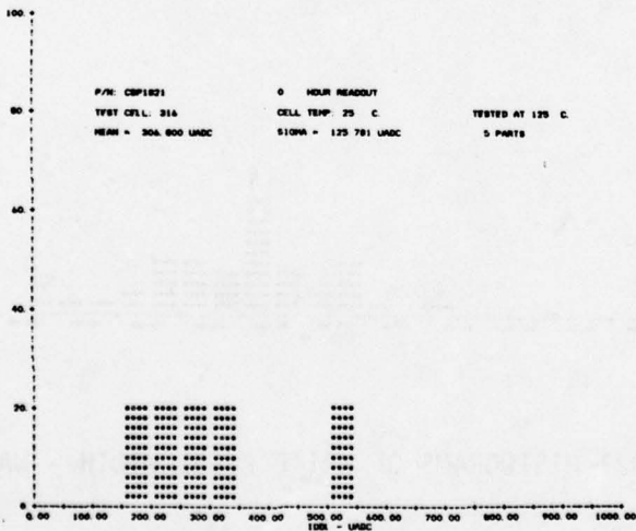
FIGURE F16. CDP1821 HISTOGRAMS OF SUPPLY CURRENT WITH V_{DD} = 5.25 VOLTS
