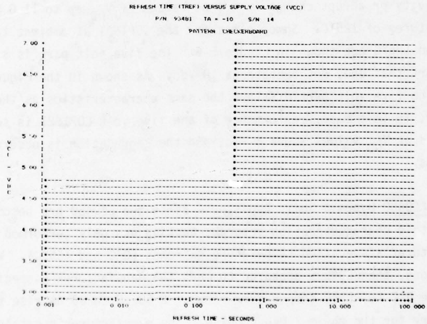
FIGURE 5-3. FAIRCHILD 93481 REFRESH TIME SHMOOS SHOWING LOW TEMPERATURE LIMITATION
