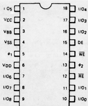
FIGURE E1. TERMINAL CONNECTION
