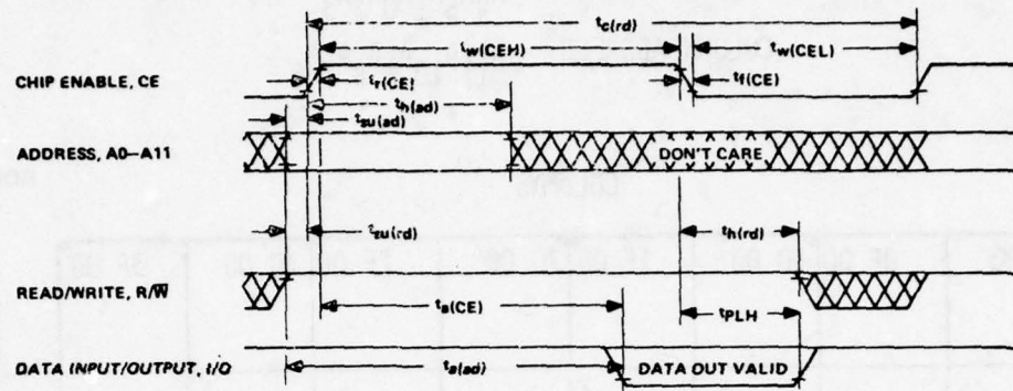
a) TIMING DIAGRAM
