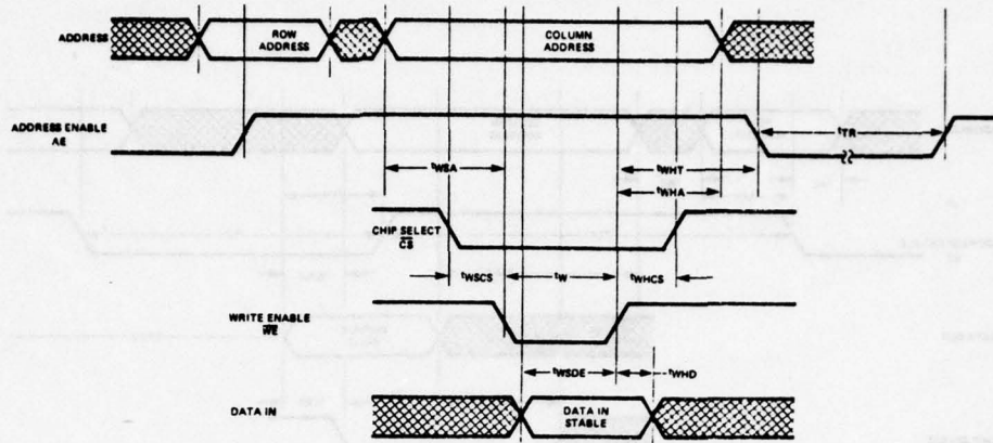
a) TIMING DIAGRAM
