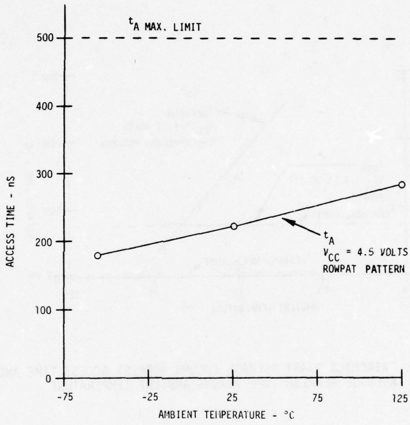
FIGURE 9-3. ADVANCED MICRO DEVICES AM9140 AVERAGE CHIP ENABLE ACCESS TIME VERSUS AMBIENT TEMPERATURE
