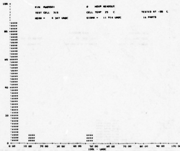
FIGURE F10. MWS5501 HISTOGRAMS OF SUPPLY CURRENT WITH V_{DD} = 5.25 VOLTS
