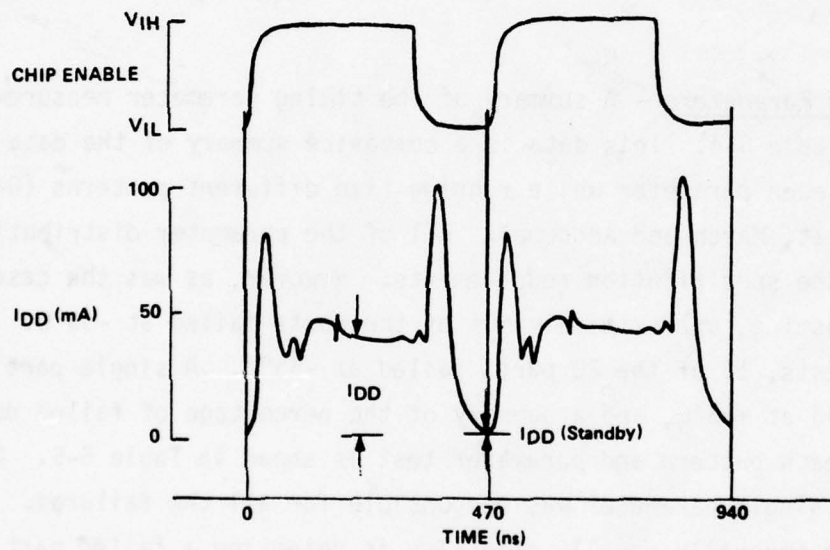
FIGURE 6-1. TEXAS INSTRUMENTS TMS4050 WAVEFORMS SHOWING STANDBY CURRENT SETTLING TIME
