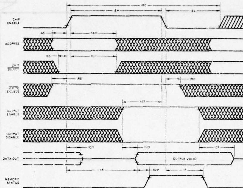
a) TIMING DIAGRAM
