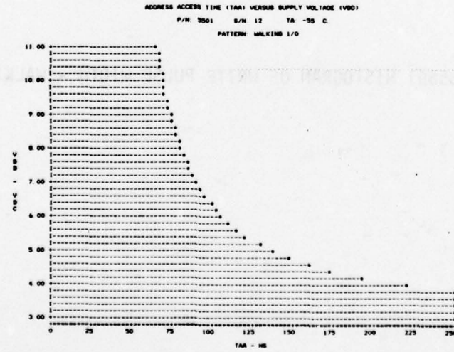
FIGURE F13. MWS5501 SHMOOS FOR ADDRESS ACCESS TIME - WALKING PATTERN
