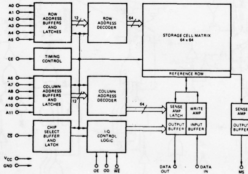
FIGURE B2. FUNCTIONAL BLOCK DIAGRAM
