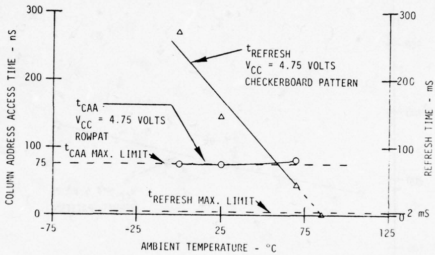
FIGURE 9-2. FAIRCHILD 93481 AVERAGE COLUMN ADDRESS ACCESS TIME AND AVERAGE REFRESH TIME VERSUS AMBIENT TEMPERATURE
