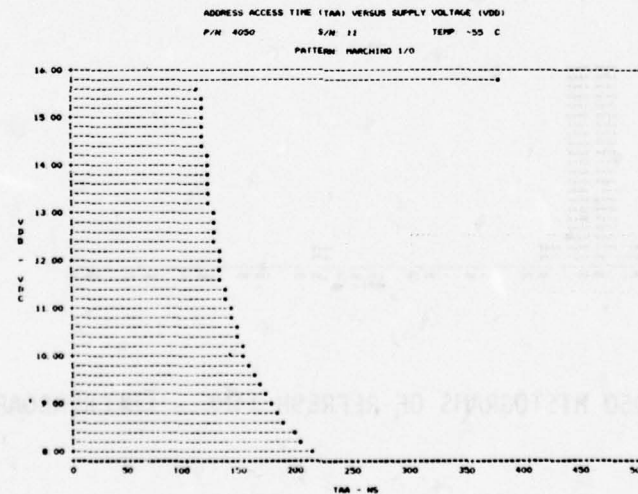
FIGURE F5. TMS4050 SMOOS FOR ADDRESS ACCESS TIME - MARCHING PATTERN
