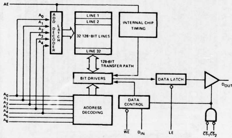
FIGURE D2. FUNCTIONAL BLOCK DIAGRAM
