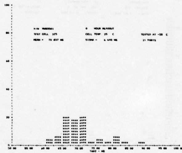
FIGURE F11. MWS5501 HISTOGRAMS OF ADDRESS ACCESS TIME - WALKING PATTERN
