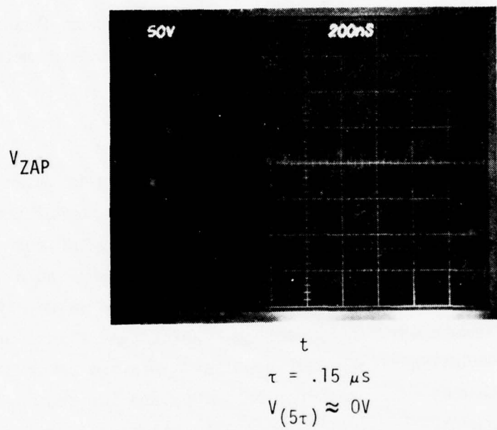
FIGURE 8-3. HIGH VOLTAGE ZAP TEST DISCHARGE VOLTAGE
