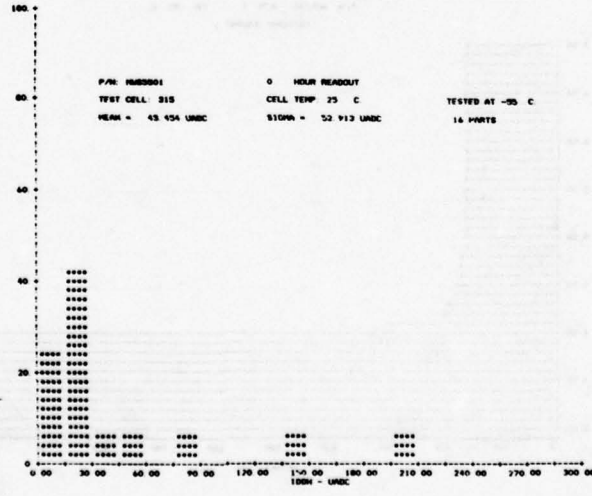
FIGURE F9. MWS5501 HISTOGRAMS OF SUPPLY CURRENT WITH V_{DD} = 10.5 VOLTS
