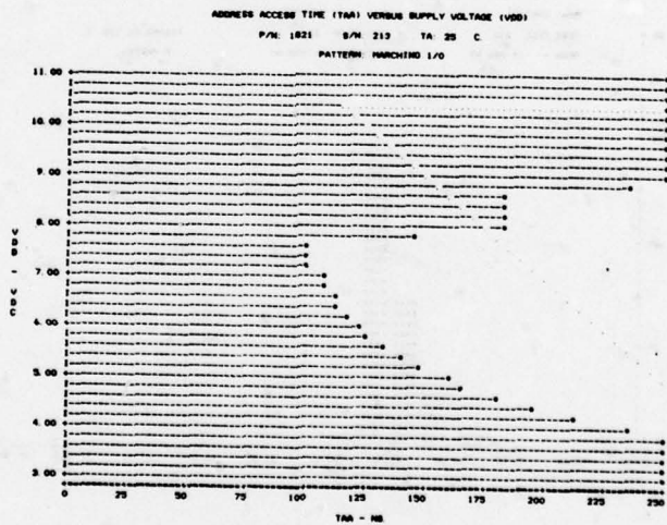
FIGURE F19. CDP1821 SHMOOS FOR ADDRESS ACCESS TIME - WALKING AND MARCHING PATTERNS
