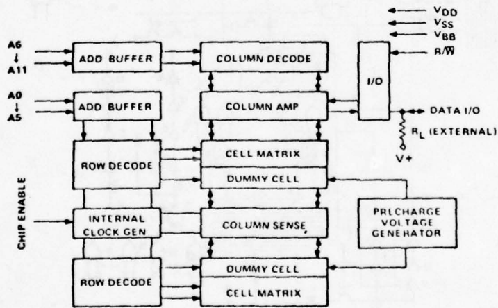
FIGURE A2. FUNCTIONAL BLOCK DIAGRAM
