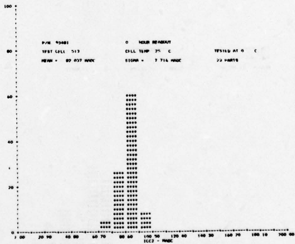
FIGURE F20. 93481 HISTOGRAMS OF SUPPLY CURRENT
