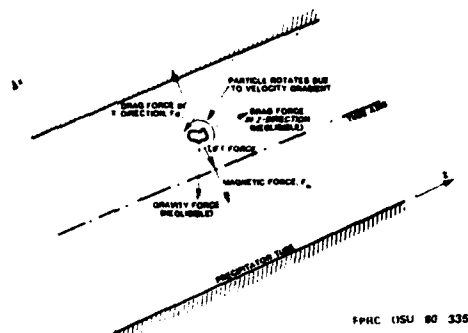
Fig. 5. Forces on the Magnetic Particle.
