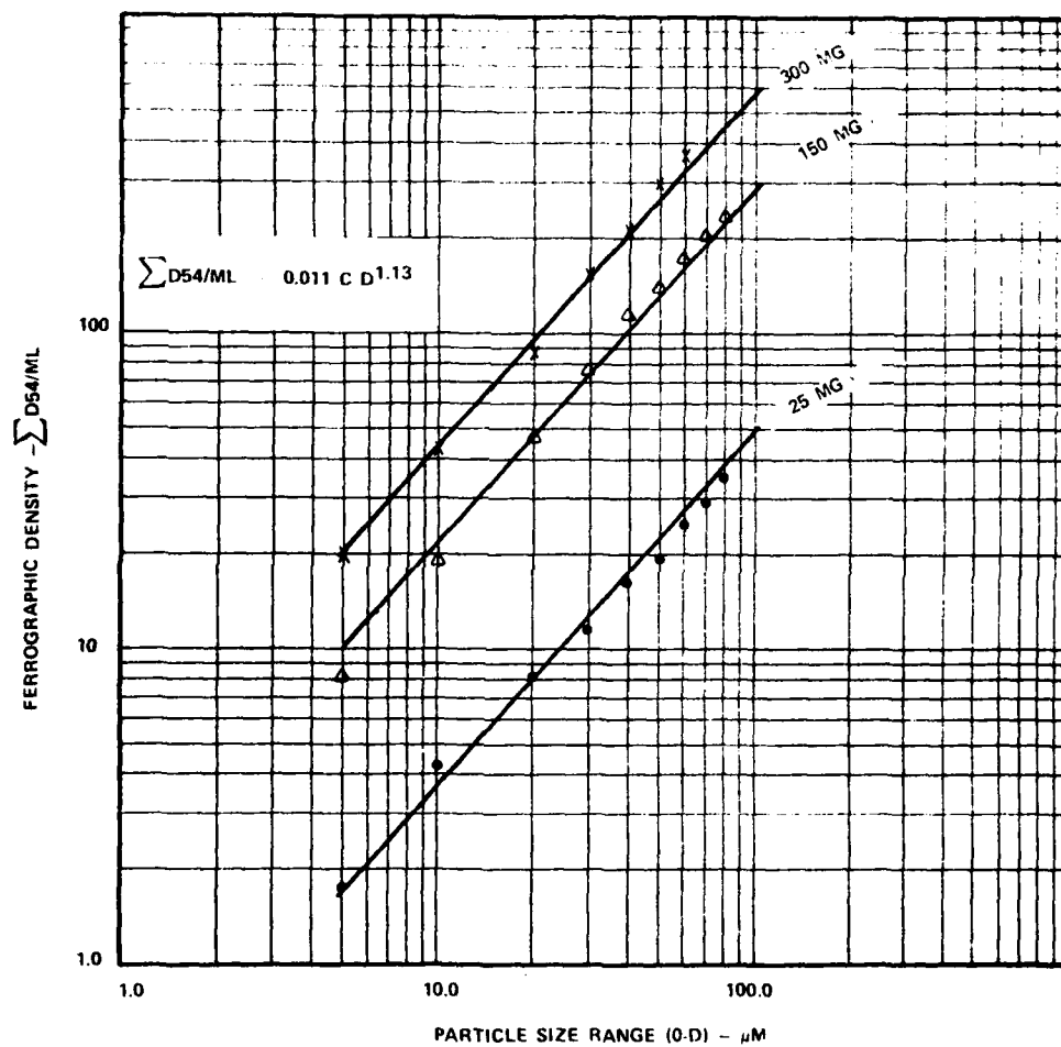
Fig. 4. Ferrographic Density vs. Particle Size Range for Various Concentrations
