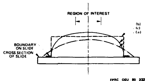
Fig. 3. Fluid Cross Section and Region of Interest.
