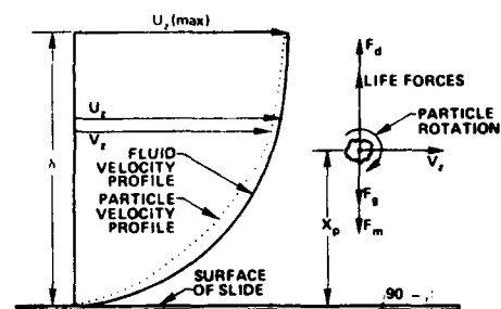
Fig. 5. Effect of Lift Force in Producing Log on Particle Velocity Profile.
