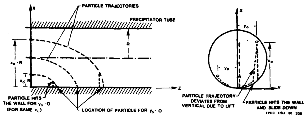
Fig. 6. Trajectory of a Particle of Given Diameter for Different Initial Position ( X_0, Y_0 ).
