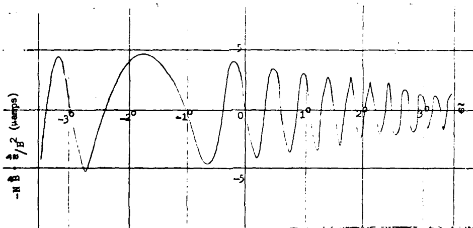
FIGURE A-11. TRANSVERSE VARIATION OF -N \mathbf{B} \cdot \mathbf{a}/B^2
