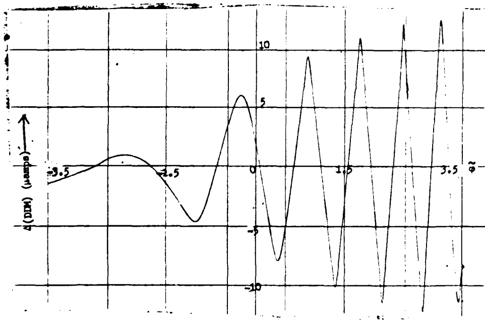
FIGURE A-7. TRANSVERSE VARIATION OF \Delta (DDM)
