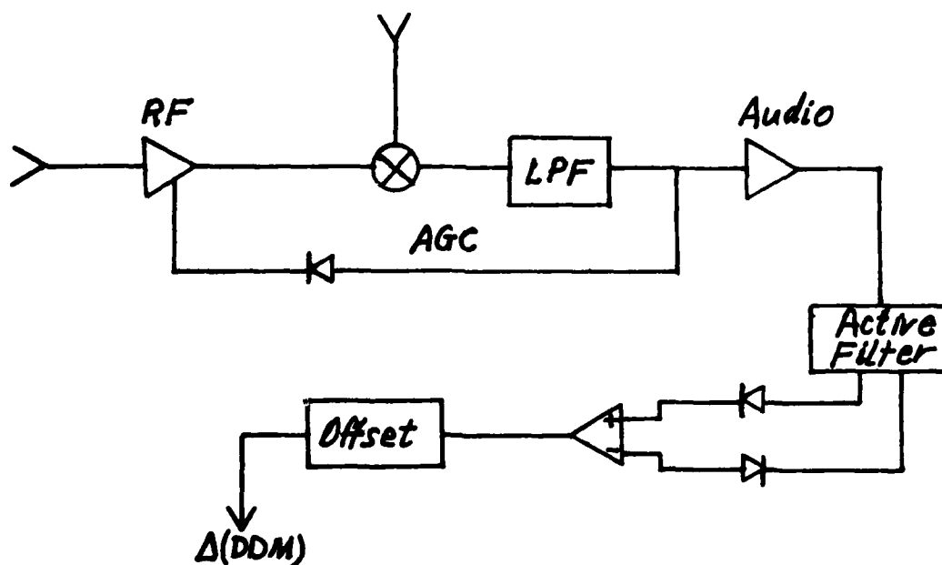
FIGURE 3-22b AM MODULE
