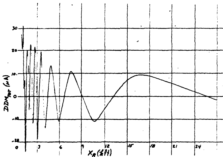
FIGURE A-47. FLIGHT PATH DIM TOT
