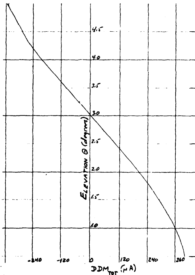
FIGURE A-41. DDM A VS. ELEVATION
