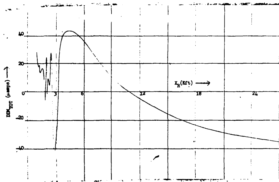
FIGURE A-13. GLIDE SLOPE Δ (DIM) VS. FLIGHT PATH GROUND COORDINATE
