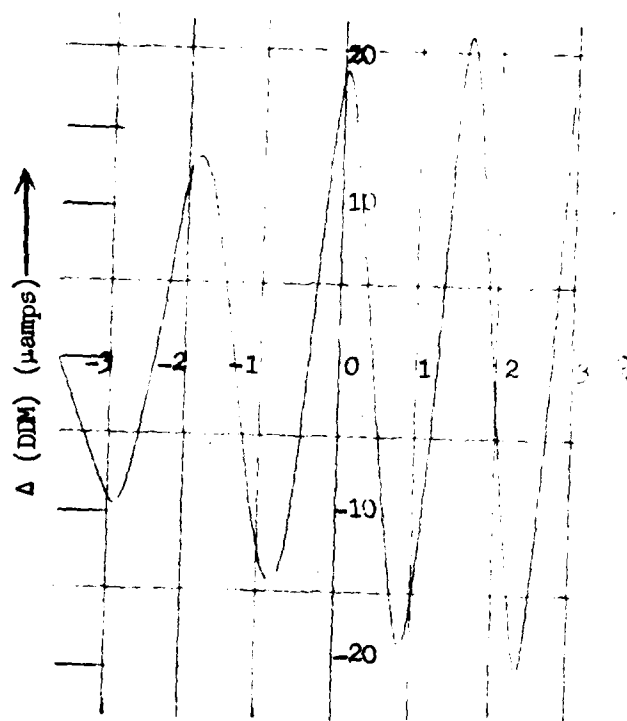
FIGURE 2-10. TRANSVERSE VARIATION OF Δ (DIM)
