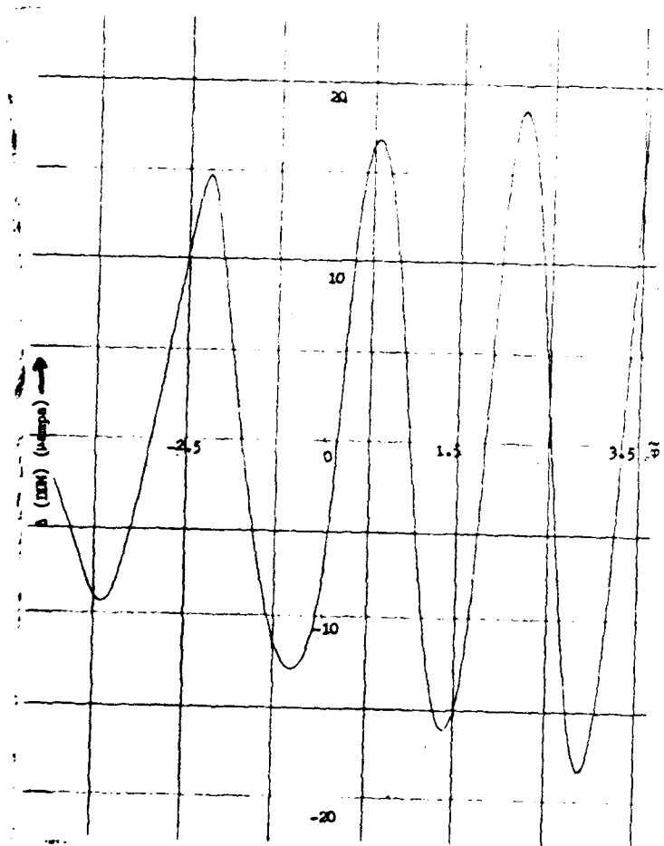
FIGURE A-9. TRANSVERSE VARIATION OF Δ (DDM)
