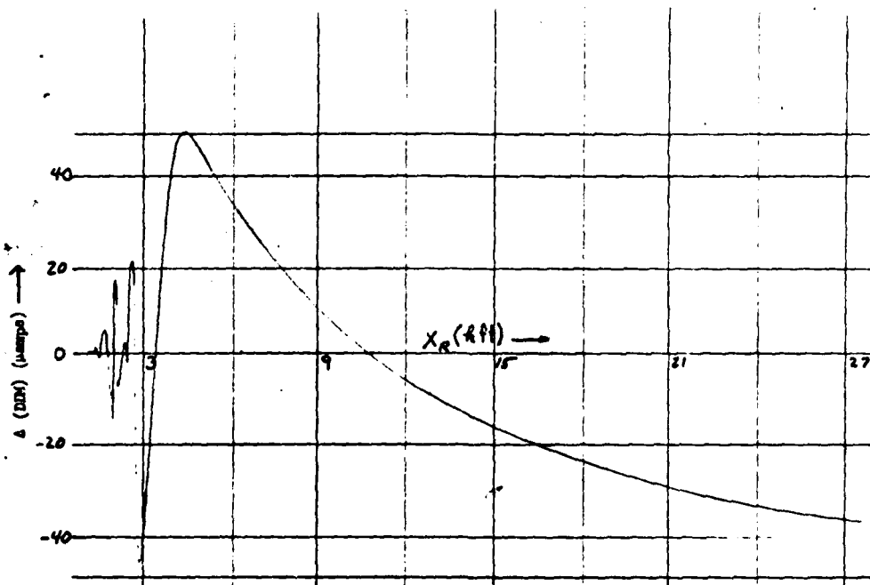
FIGURE A-14. GLIDE SLOPE DM_{TOT} VS. FLIGHT PATH GROUND COORDINATE
