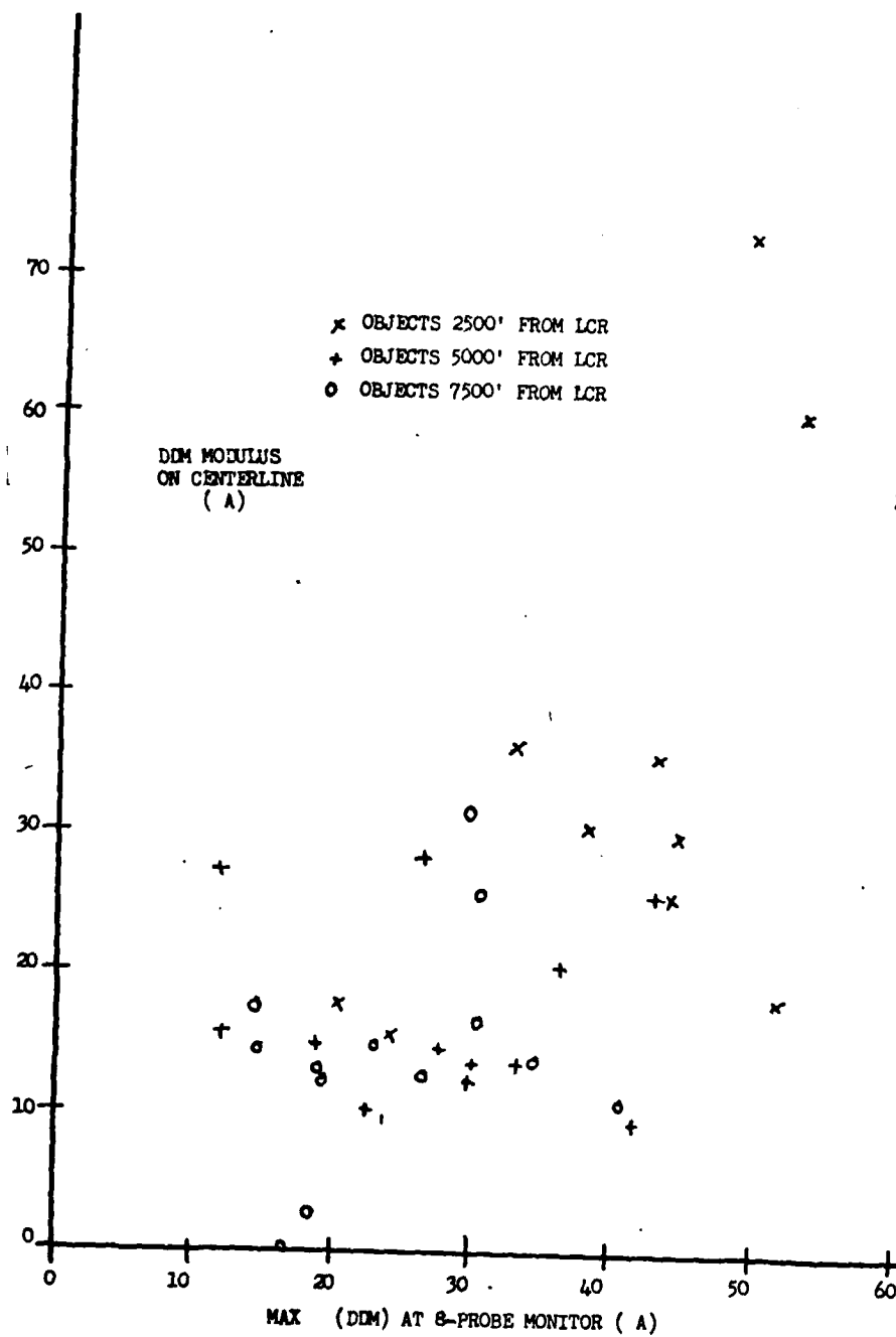
FIGURE 3-2. SCATTER DIAGRAM
