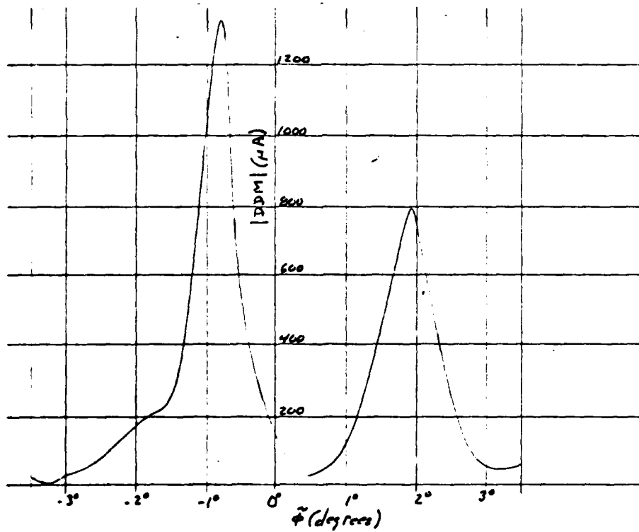
FIGURE A-36. TRANSVERSE VARIATION OF (DDM) (FLYOVER)
