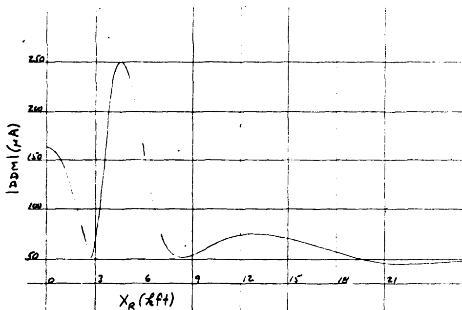
FIGURE A-38. |DDM| (FLYOVER)
