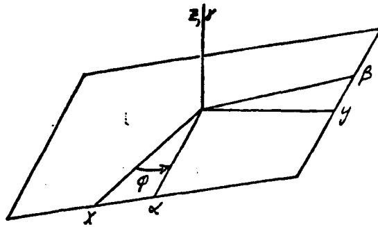
FIGURE A-4 EULER ANGLES \varphi , \varepsilon , \chi
