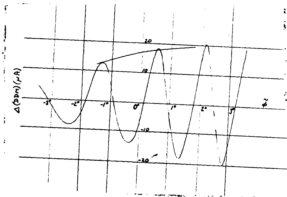
FIGURE A-16. TRANSVERSE VARIATION OF \Delta (DDM)
