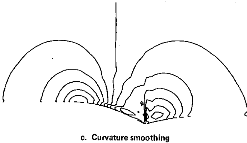
Figure 4. Effect of third-order smoothing.
