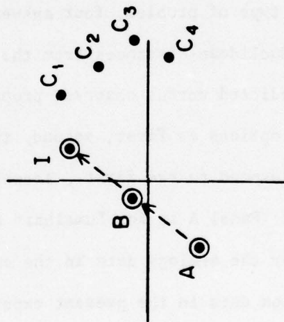
Series Completion
