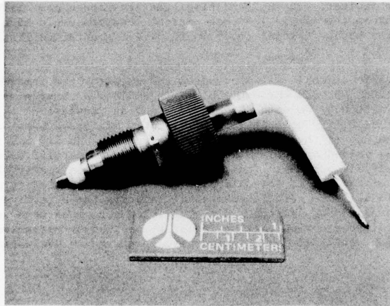
Figure 87. Spark Plug High-Voltage Cable Connector
