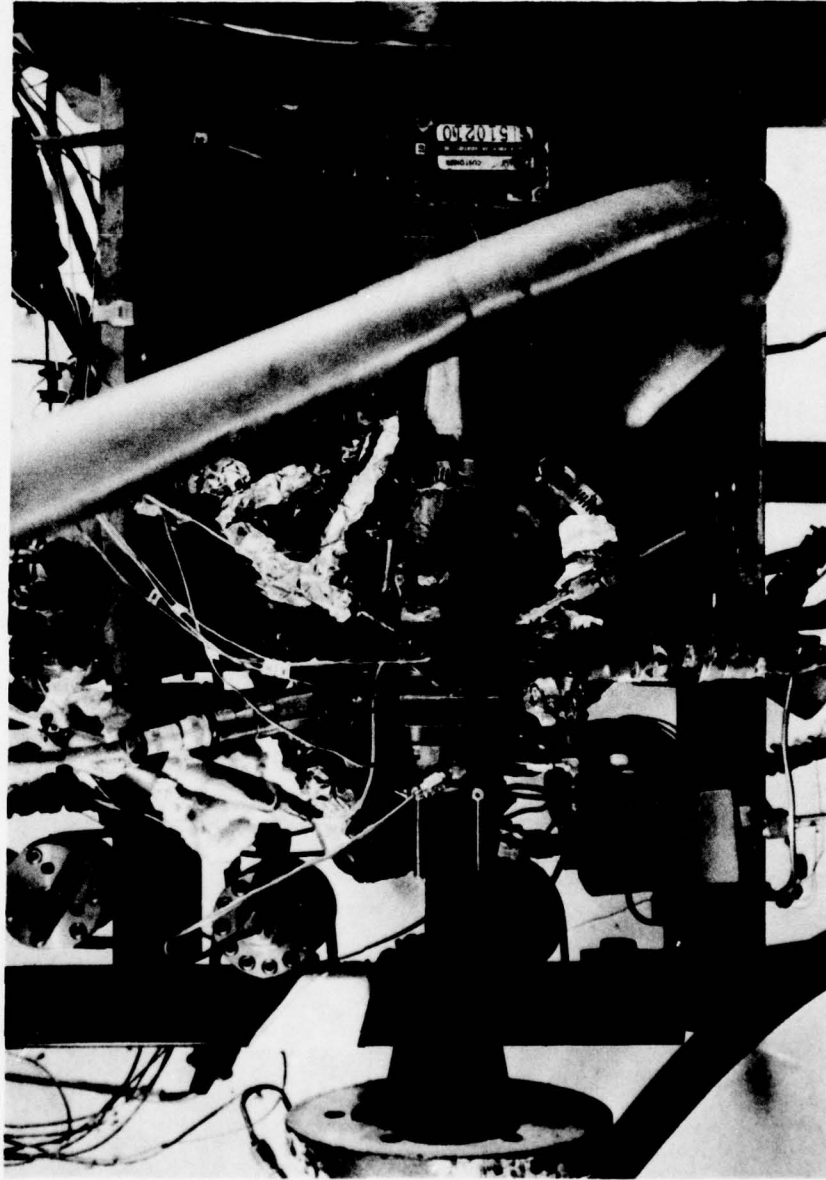
Figure 80. Installation of Durak "B" Coated Molybdenum Thrust Chamber With the BLH Load Cell
