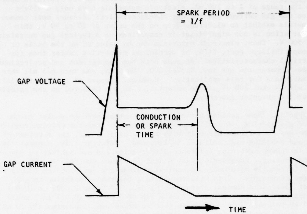
TYPICAL INDUCTIVE WAVEFORM
