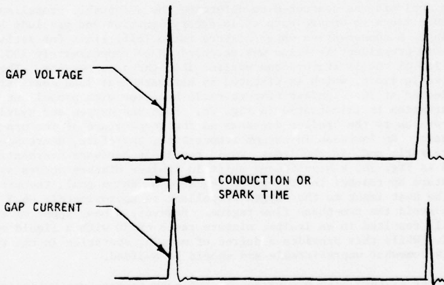
TYPICAL CAPACITIVE WAVEFORM
