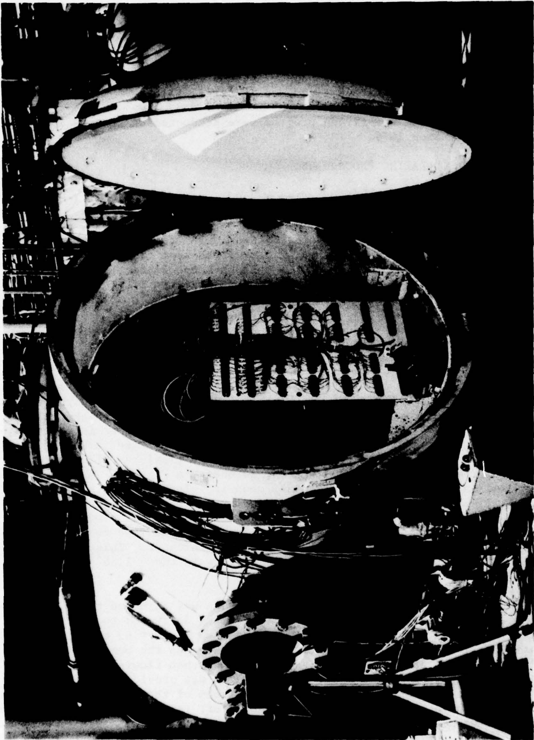
Figure 75. Overall View of 25-pound Thruster Test Facility
