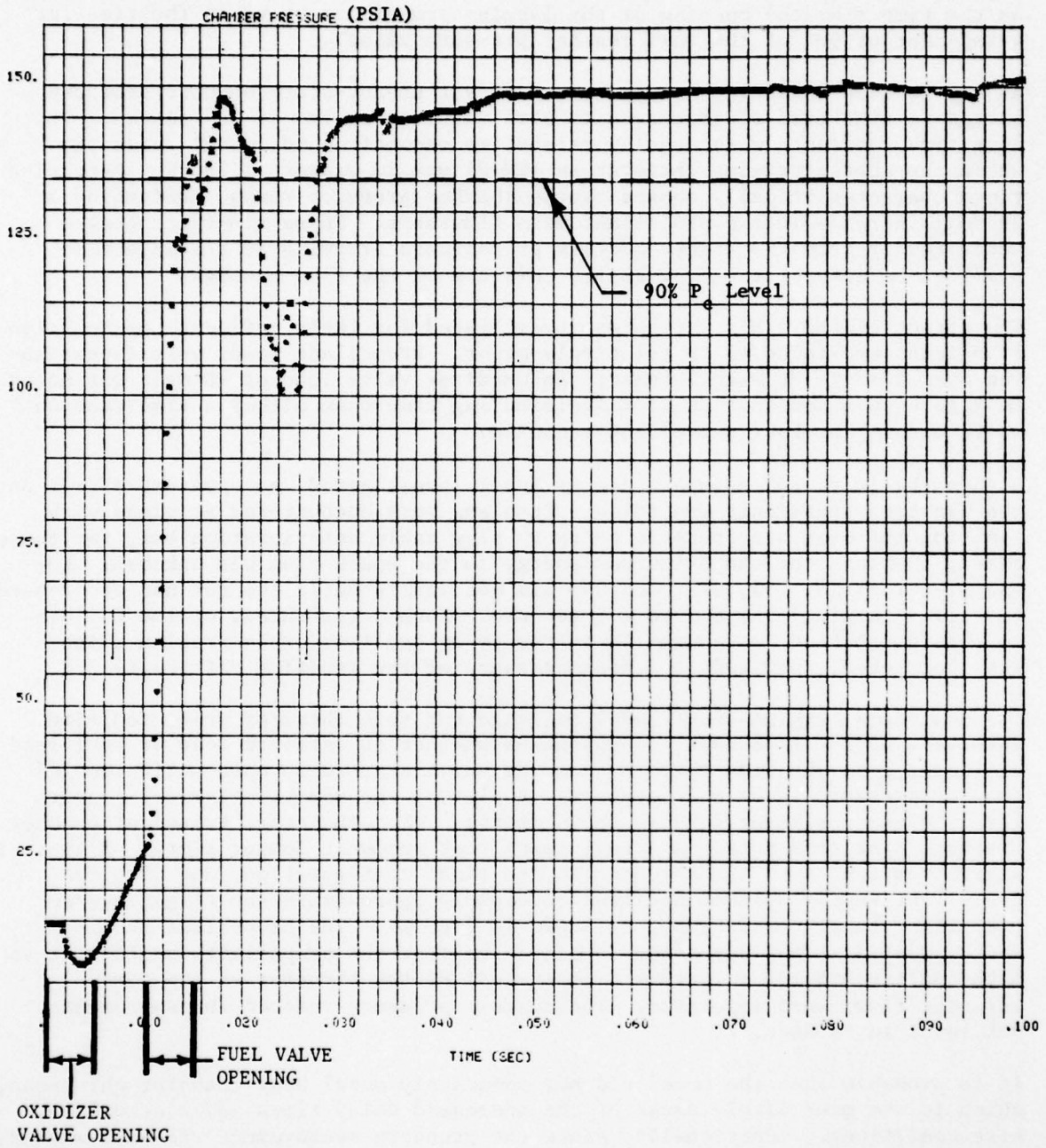
Figure 97. Predicted Chamber Pressure Behavior With Time
