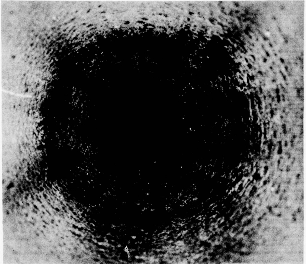
Figure 96. Thrust Chamber Throat Erosion Viewed From Exit End of Nozzle (Posttest 071)
