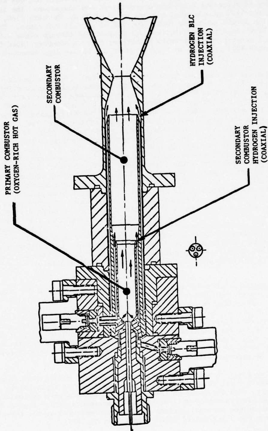
Figure 88. Baseline Thruster Configuration
