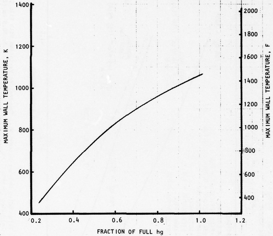
Figure 47. Injector Region Maximum Wall Temperature Variation With Heat Transfer Coefficient ( MR_{Core} = 50:1 )
