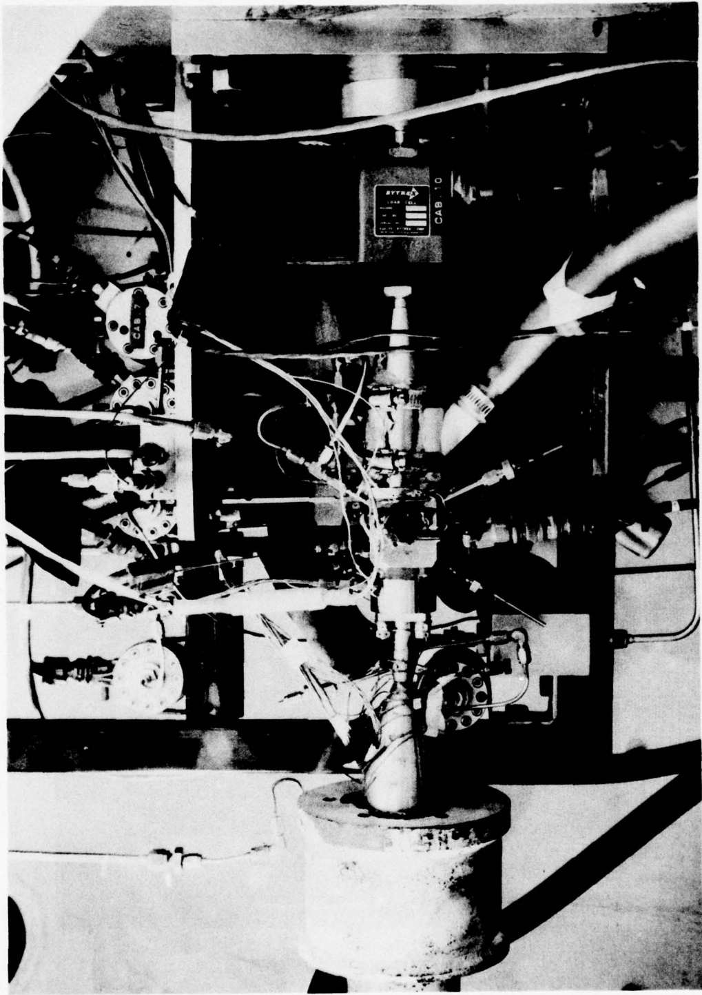
Figure 79 . Thruster Installation With Provisions for Pressurization of High-Voltage Spark Plug Cable
