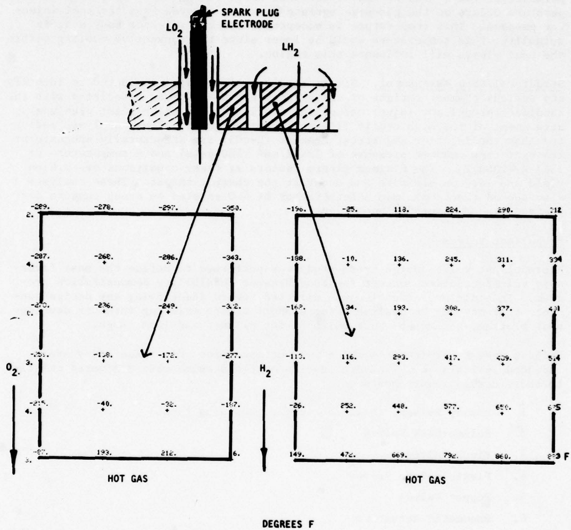
Figure 48. Injector Region Temperature Distribution (0.5 hg and MR_{core} = 50:1 )
