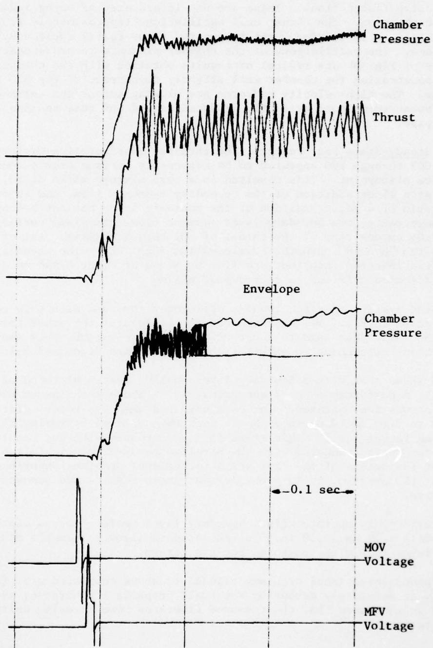
Figure 98. Thruster Start Transients for Run No. 93 (Oscillograph Tracings)
