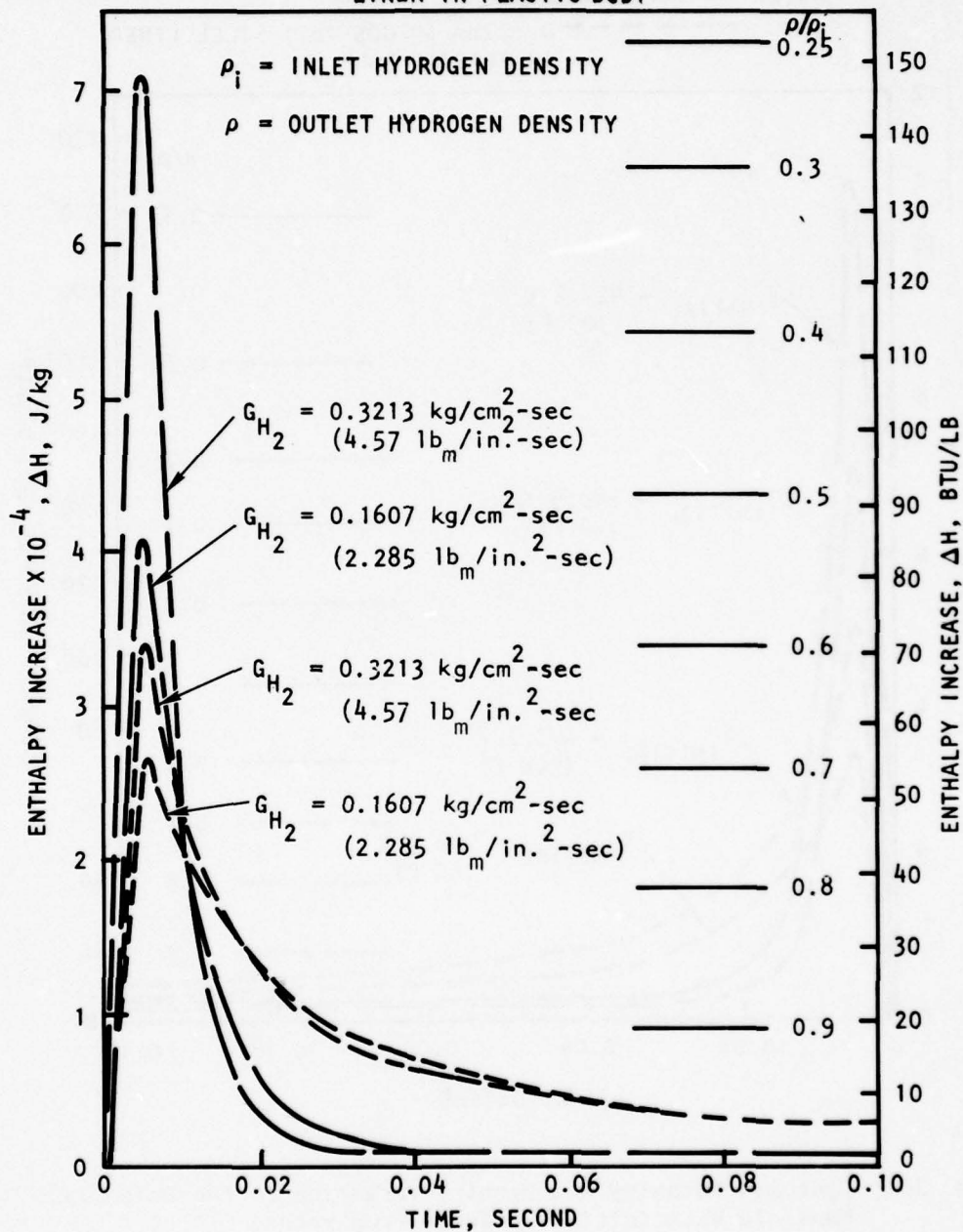
Figure 19. Hydrogen Enthalpy and Density Variation With Flowrate
