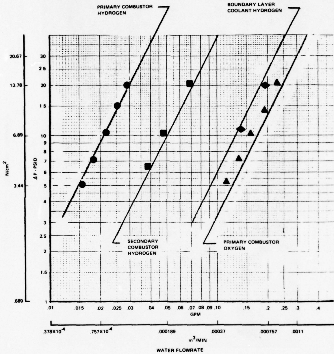
Figure 74. Thruster Hydrogen Circuit Flow Characteristics
