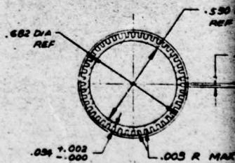
VIEW EE
