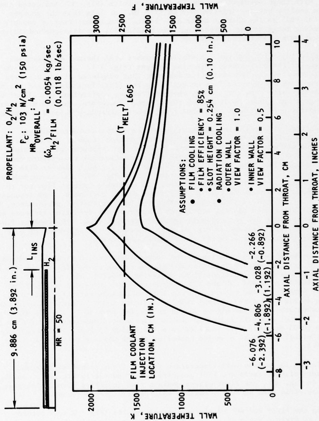
Figure 31. Chamber Wall Temperature Variation With Film Coolant Injection Location (Single Fuel Sleeve Design)
