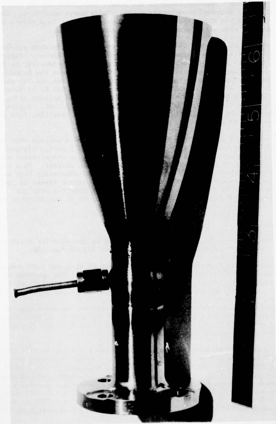
Figure 95. External Surface Heat Discoloration Pattern Shown Posttest 071
