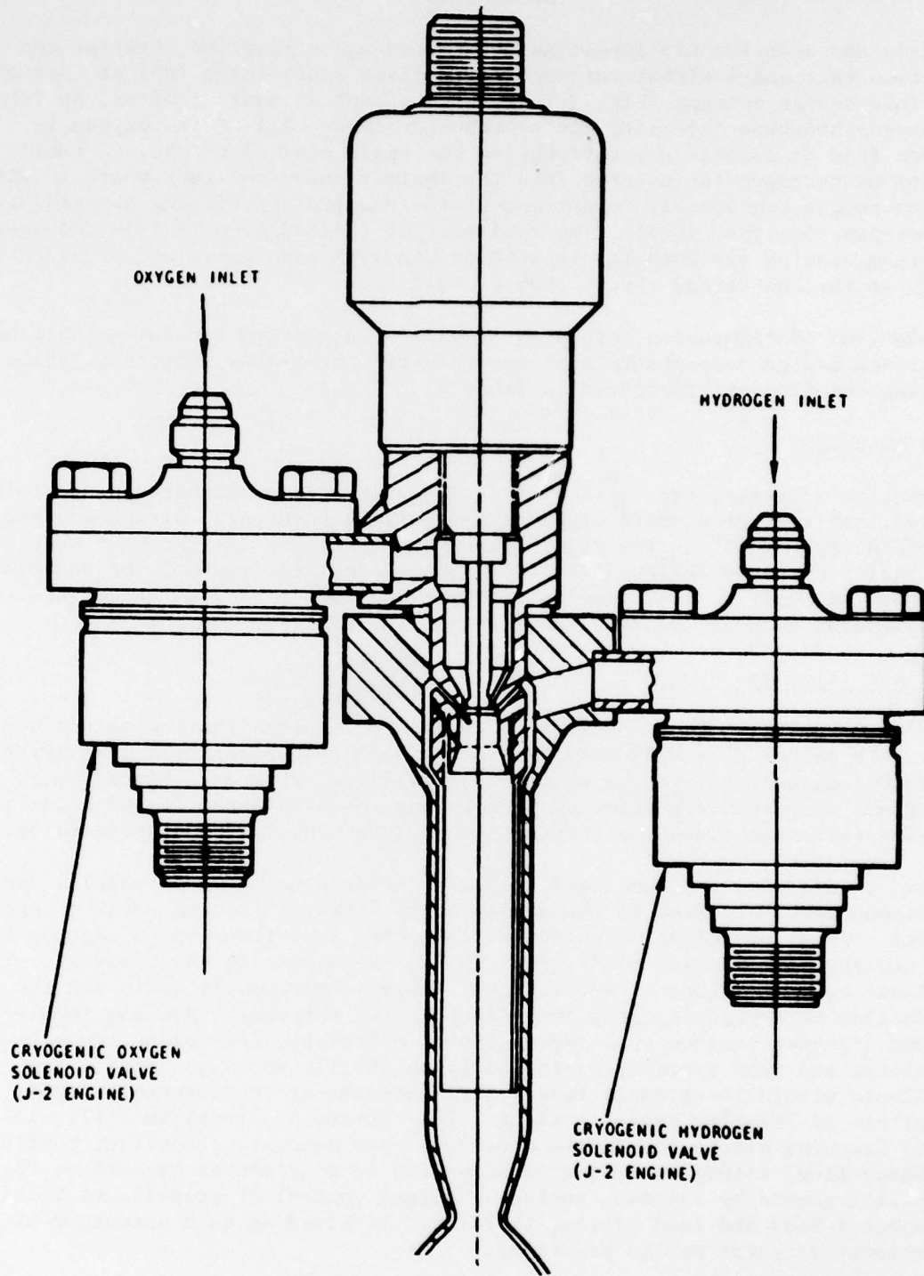
Figure 1 . Baseline Thruster Concept
