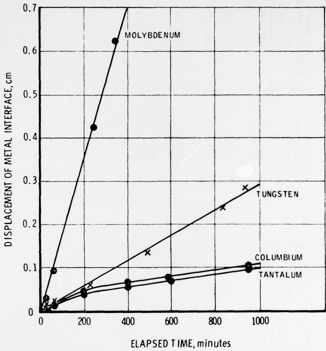
Figure 62 . Oxidation of Mo, Ta, and Cb in Flowing Air at 1367 K (2460 R)
