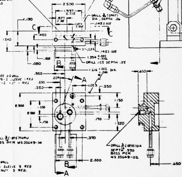
DETAIL OF PROPELLANT FEED SYSTEM NOZZLE SUPPORT
