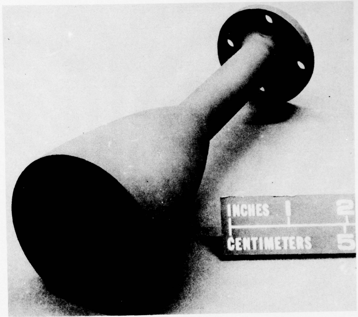
Figure 70. Thrust Chamber Assembly (Molybdenum)
