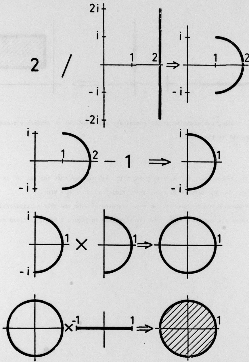
Figure 5. How to produce the unit circle and the unit disc from numbers and segments using arithmetic operations.
