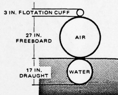
Boom structure
