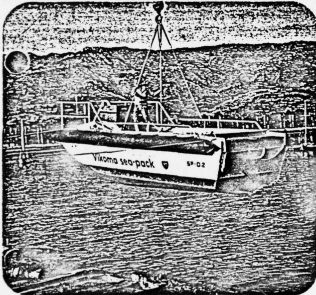
SEAPACK being lowered into water by its own lifting strrops.
