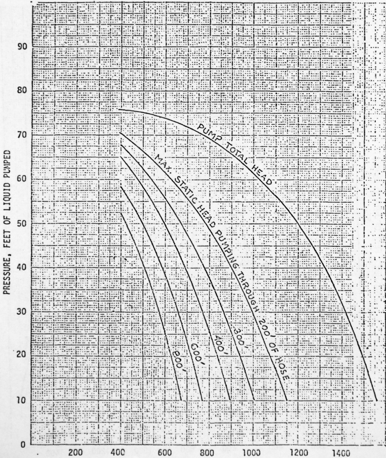
FIGURE E-3 SUBMERSIBLE PUMP AND TRANSFER HOSE PERFORMANCE CHARACTERISTICS (AT PUMP RATED SPEED - 1750 RPM) BUNKER "C" (700 S.S.U. @ 130 °F)
