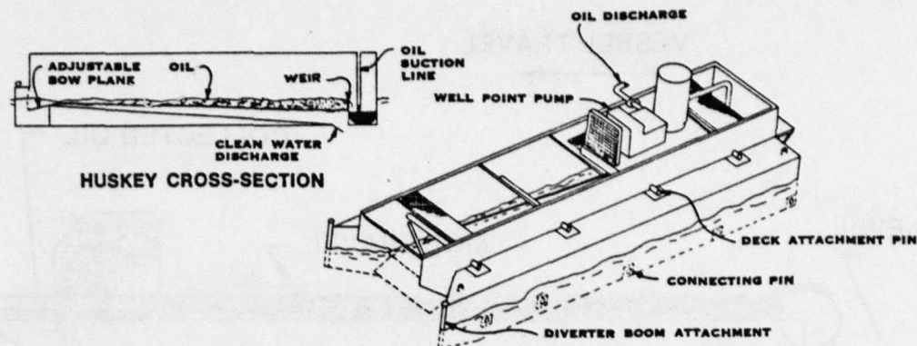
HUSKEY OFFSHORE SKIMMER
