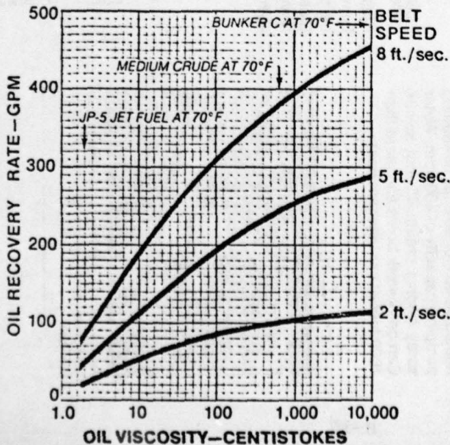
Oil recovery rate for a 3' wide Filterbelt
