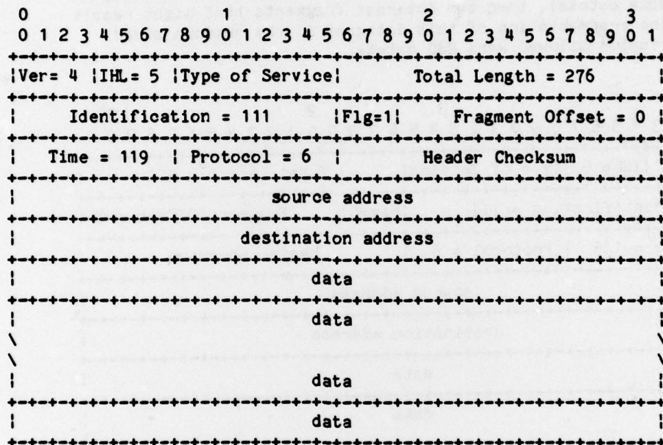
Example Internet Fragment
