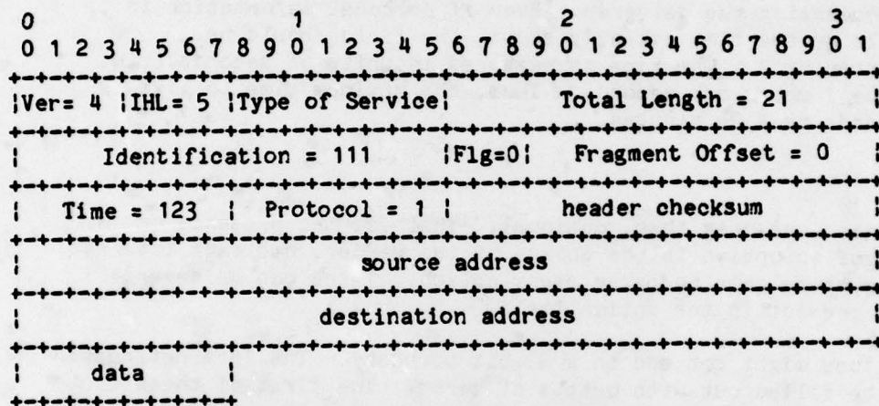
Example Internet Datagram
