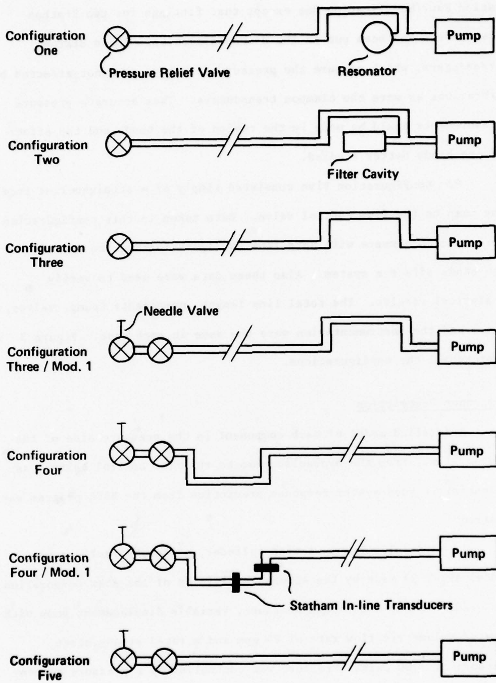
Figure 3. Line Configurations
