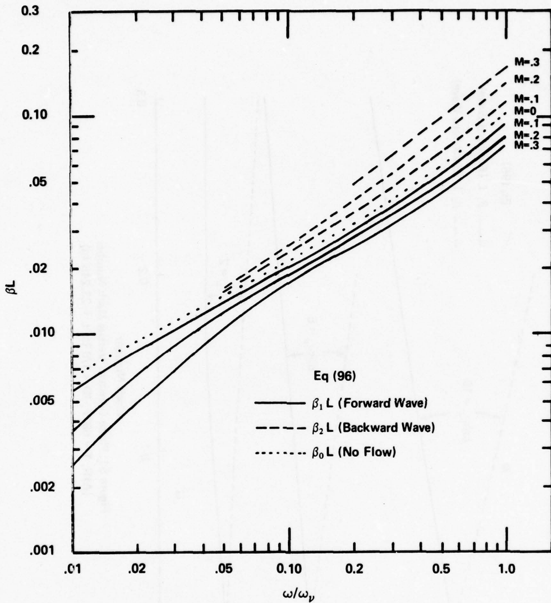
Figure 50. Phase Constant for Small Frequency Ratios (AIR, T = 59°F, ID = 1/8 In, L = 23.245 In)
