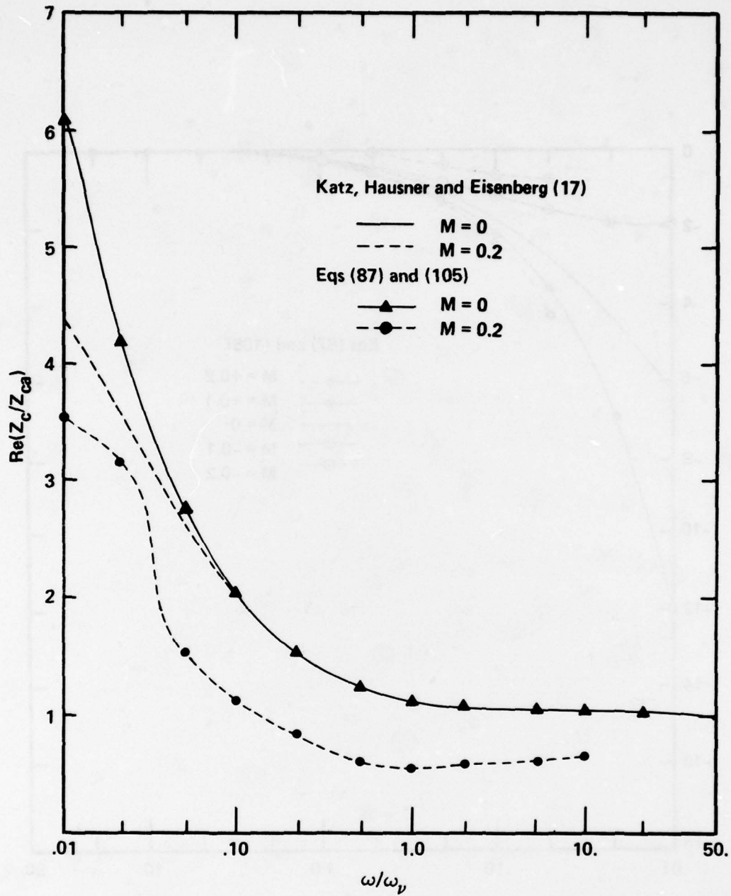
Figure 69. Real Part Of The Normalized Characteristic Impedance For M = 0 And 0.2 Versus \omega/\omega_p
