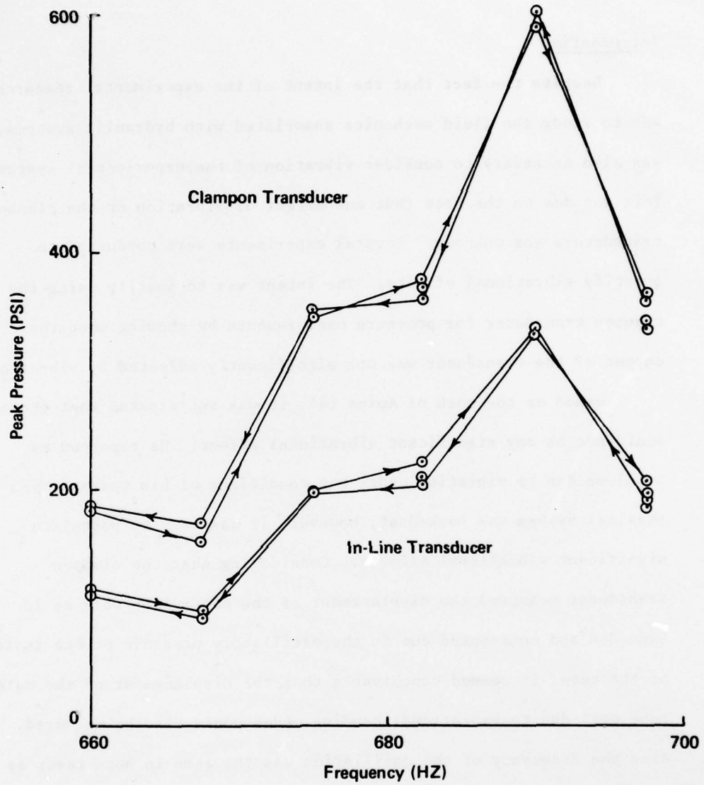
Figure 6. Repeatability Of Data Clampon Transducer 64.5 In. From Pump In-Line Transducer 101.5 In. From Pump
