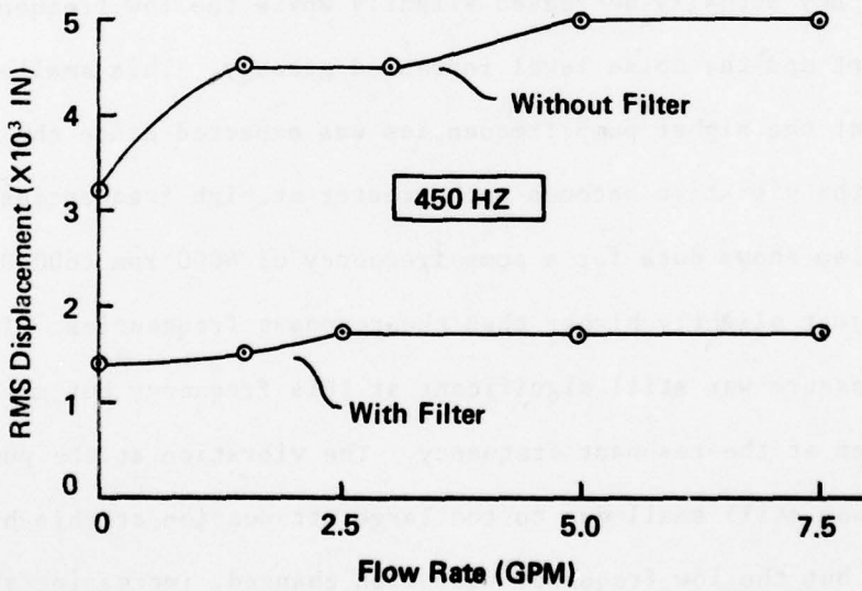
Figure 8. Vibration Displacement Measurements At 300 and 450 Hz With and Without an 110 Hz High-Pass Filter
