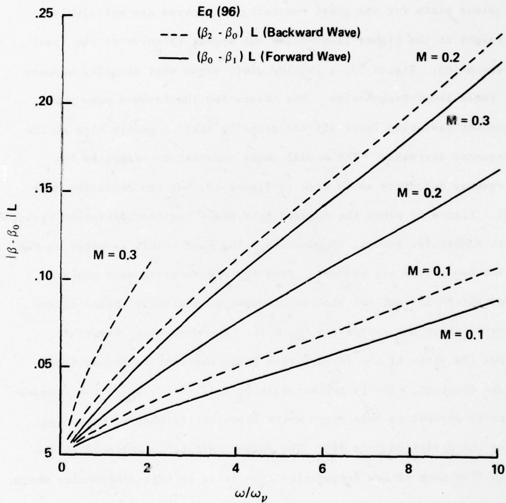
Figure 52. Phase Constant Deviation Versus \omega/\omega_p (AIR, T = 59° F, ID = 1/8 In, L = 23.245 In)
