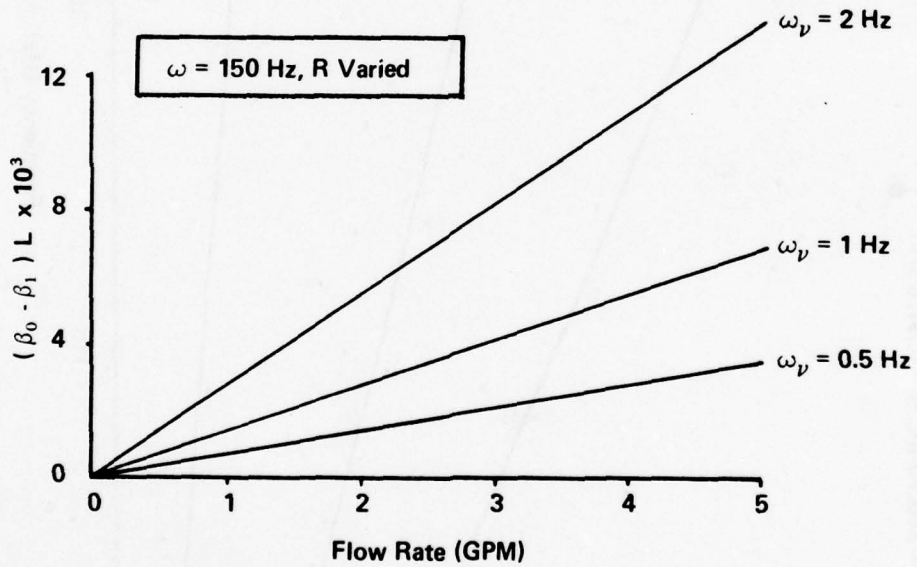
Figure 33. Effect of \omega_\nu on Phase Constant Deviation (Hydraulic Fluid, L = 209.75 \text{ In} )
