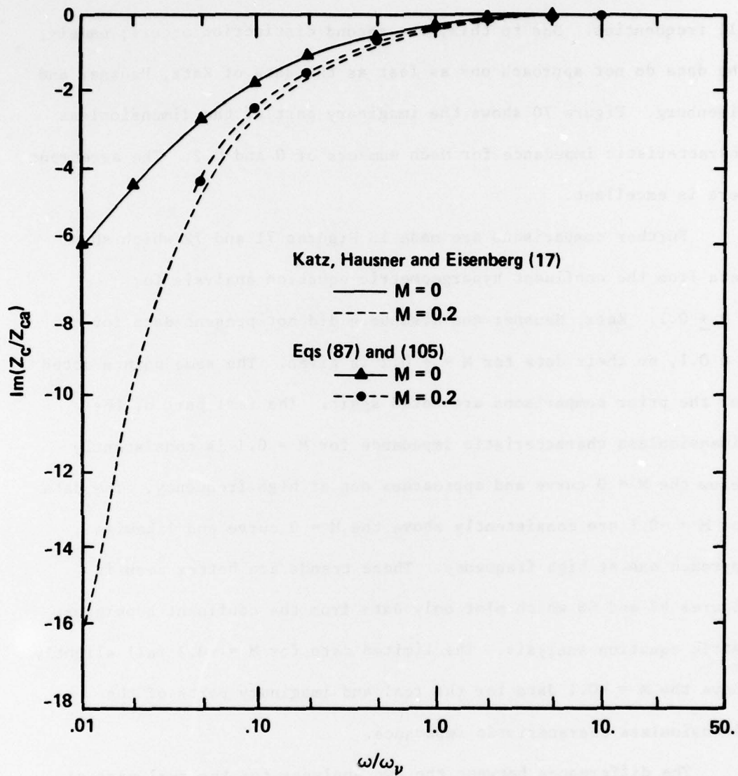
Figure 70. Imaginary Part Of The Normalized Characteristic Impedance For M = 0 and 0.2 Versus \omega/\omega_v
