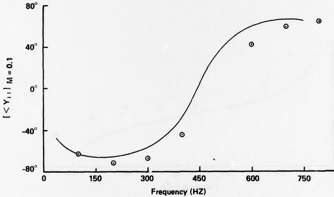
Figure 65. Comparison Of The Analytical And Experimental Values Of The Forward Driving Point Admittance For M = 0.1
