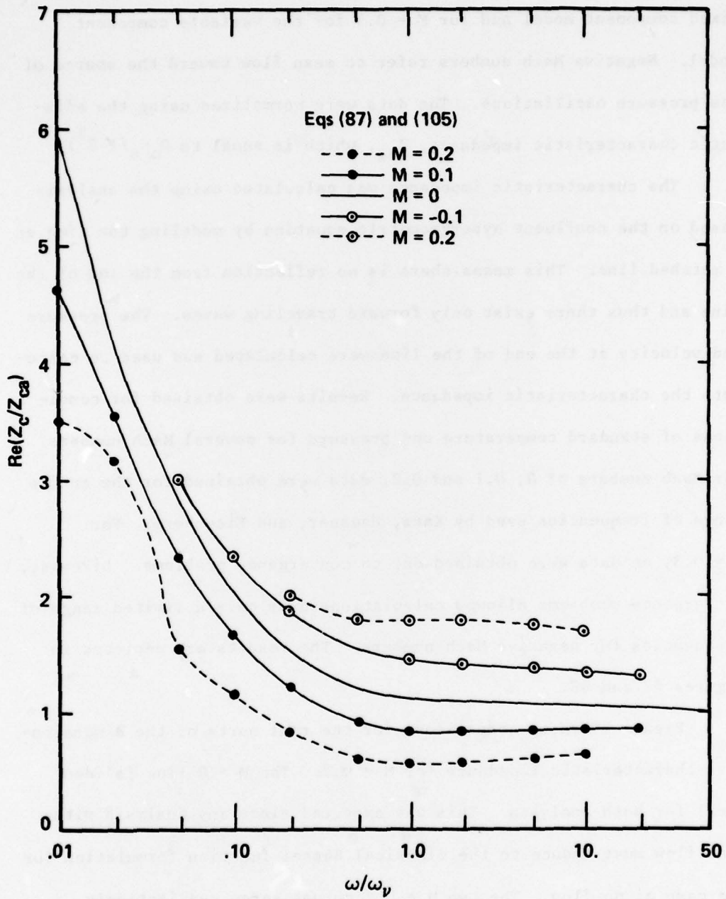
Figure 67. Real Part Of The Normalized Characteristic Impedance Versus \omega/\omega_\gamma
