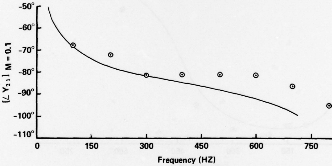
Figure 66. Comparison Of Analytical And Experimental Values Of The Forward Transfer Admittance For M = 0.1
