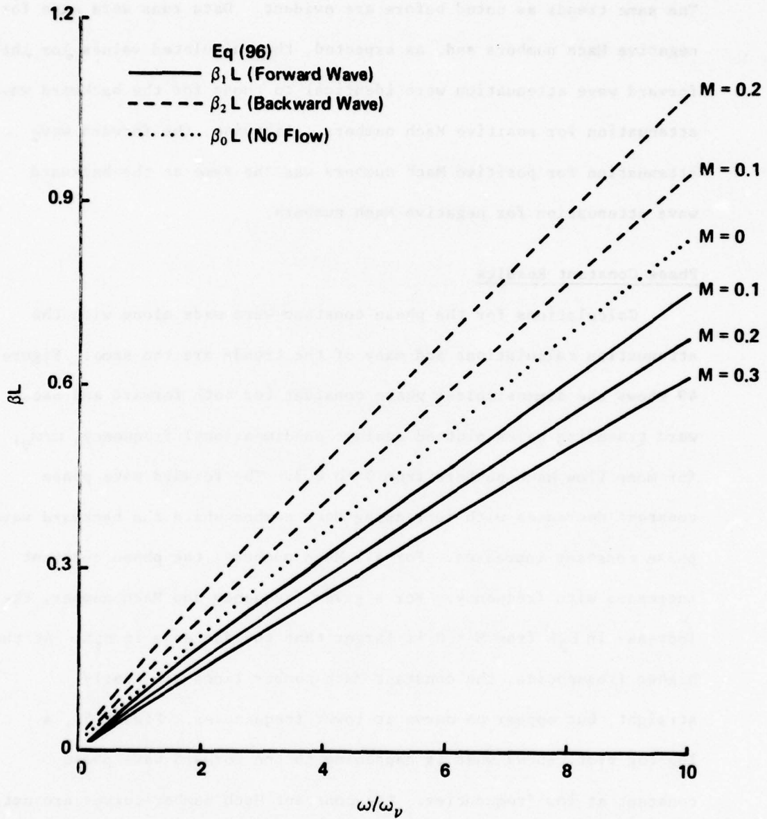
Figure 49. Phase Constant Versus \omega/\omega_v , For Mach Numbers From 0 to 0.3 (AIR, T = 59°F, ID = 1/8 In, L = 23.245 In)
