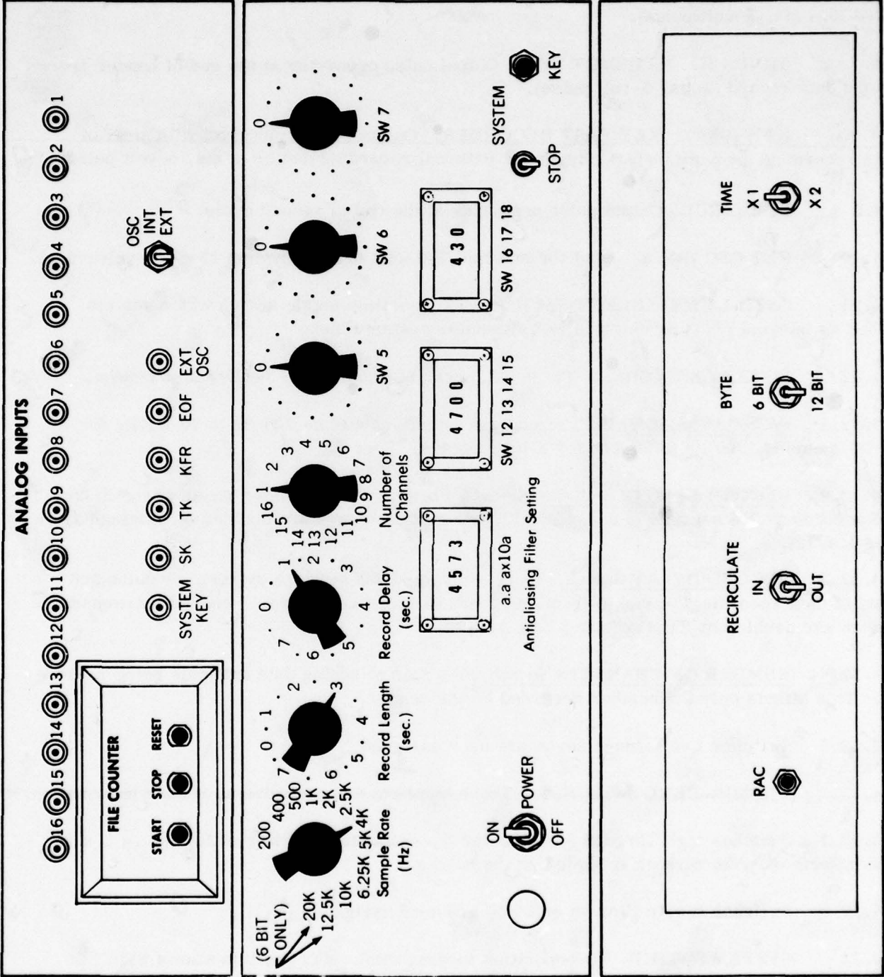
Figure 2. SDAS Front Panel
