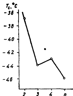
Fig. 17. Dependence T_c on a quantity of \text{CH}_2 -group in the glycol segment of polyurethane chain.
