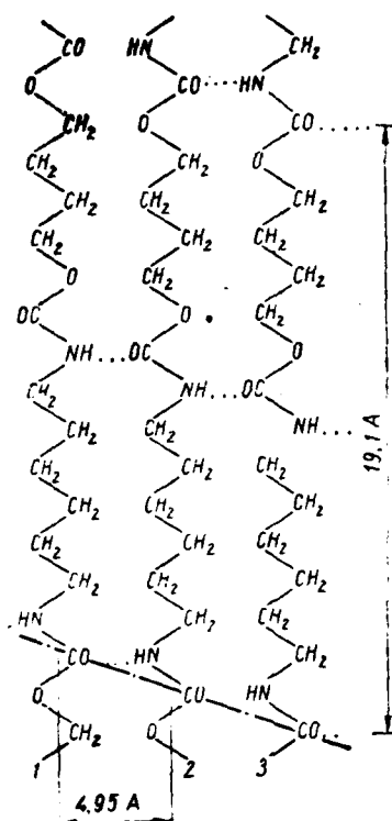
Fig. 25. Structure of the "flat/plane grid" of 4,6-polyurethane.
