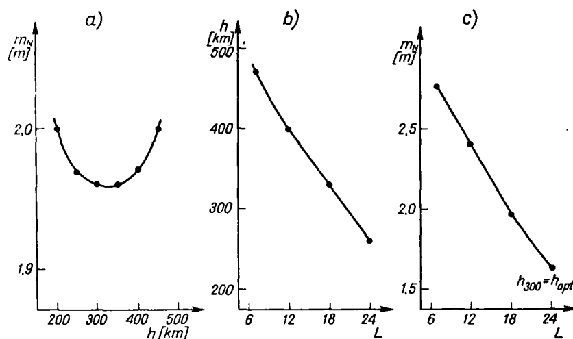
Fig. 3. a. Optimal satellite height for reference field L = 18 (share of gravimetric observations); b. Dependence of optimal height on degree and order of reference field (share of gravimetric observations); c. Accuracy of geoid undulation determination from observations at 300 km height and at optimal height as a function of degree and order of reference field (share of gravimetric observations).
