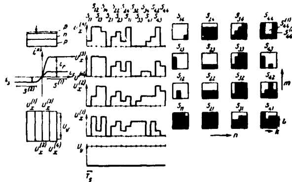
Figure 4. Dynamics of the formation of masks on photoreceiving matrix in Figure 3: a) potential-current characteristics of illuminated nonsymmetrical p-n-p (n-p-n) structure and markers of time intervals; b) graphs of potentials exciting the verses and bringing potentials to the divider; c) the corresponding profile masks of photosensitivity synthesized in the receiver panel
