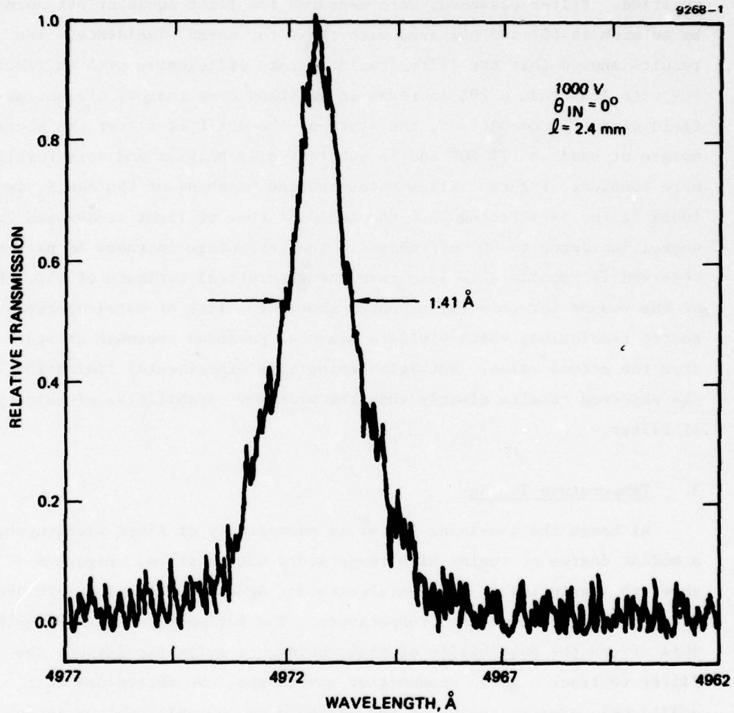
Figure 5(a). Passband of 2.4-mm-long \text{AgGaS}_2 sample: normal incidence.
