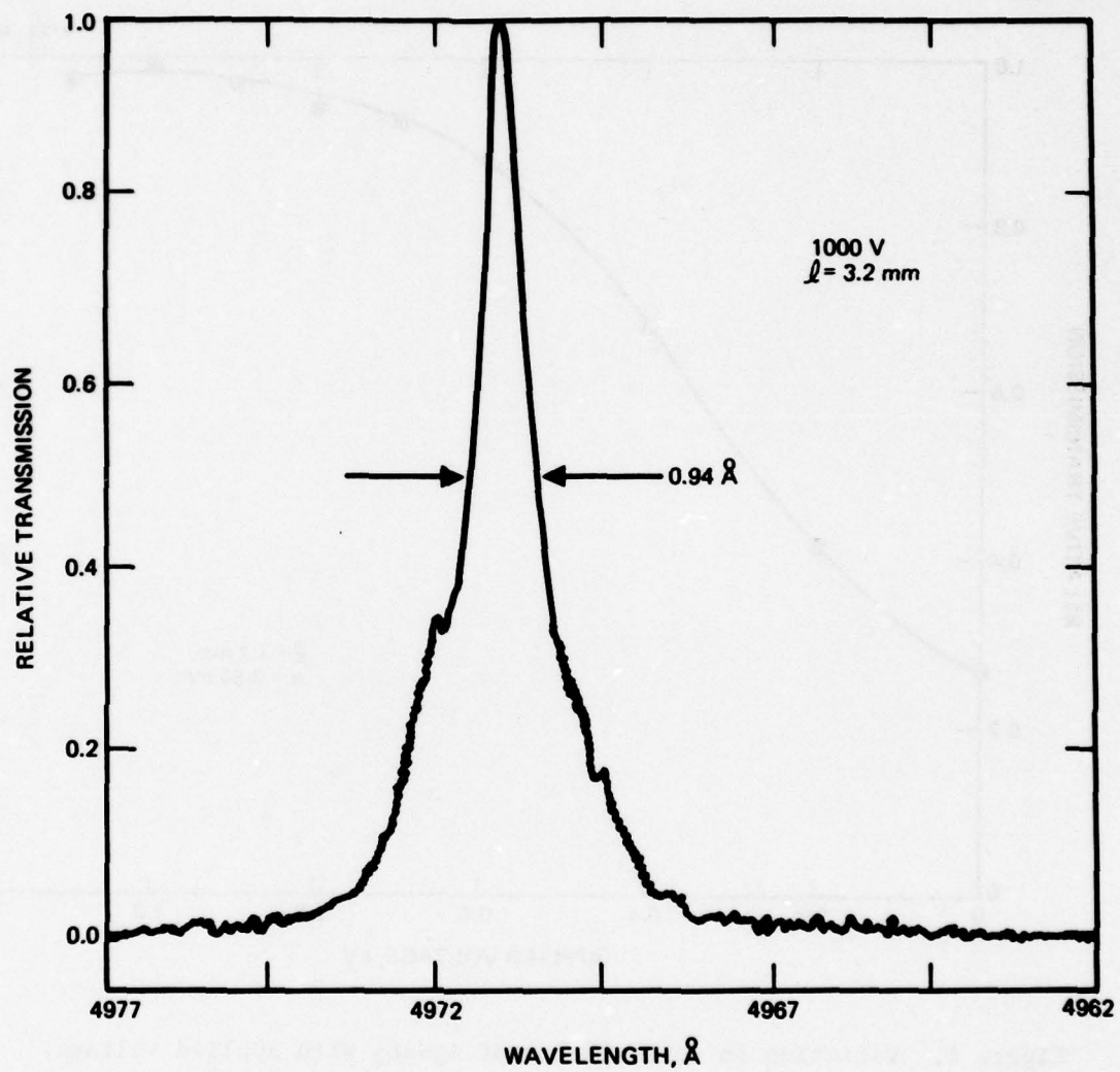
Figure 3(b). Iso-index AgGaS 2 filter transmission for a 3.2 mm sample, 1000 V applied.
