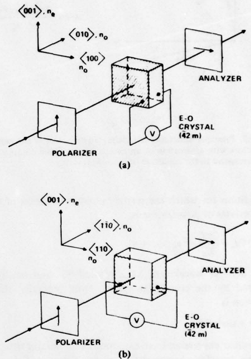
Fig. 1. Coupled-wave electrooptic filter configurations. (a) longitudinal field and (b) transverse field.
