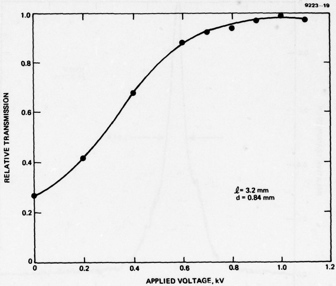
Figure 4. Variation in transmission of \text{AgGaS}_2 with applied voltage. Sample thickness d = 0.84 mm; length l = 3.2 mm.
