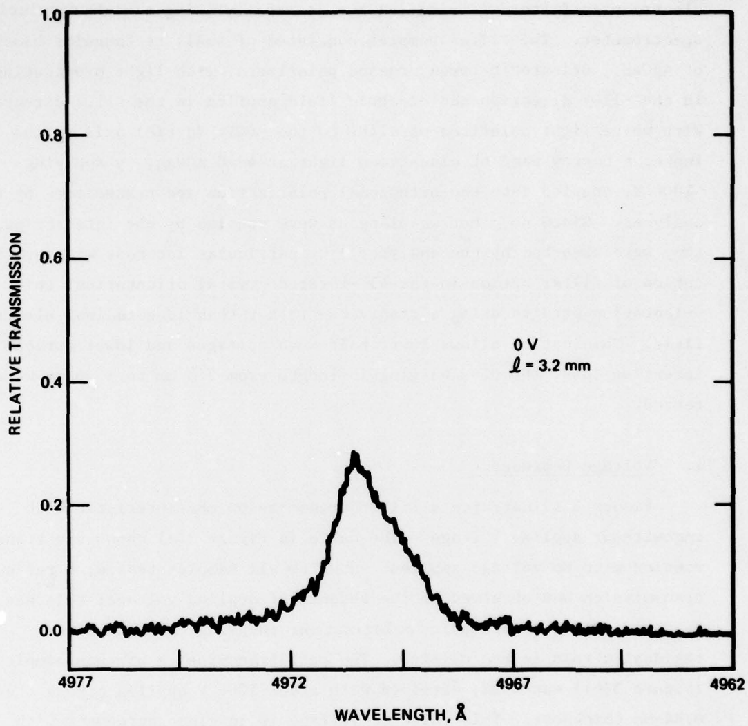
Figure 3(a). Iso-index AgGaS 2 filter transmission for a 3.2 mm sample, 0 V applied.
