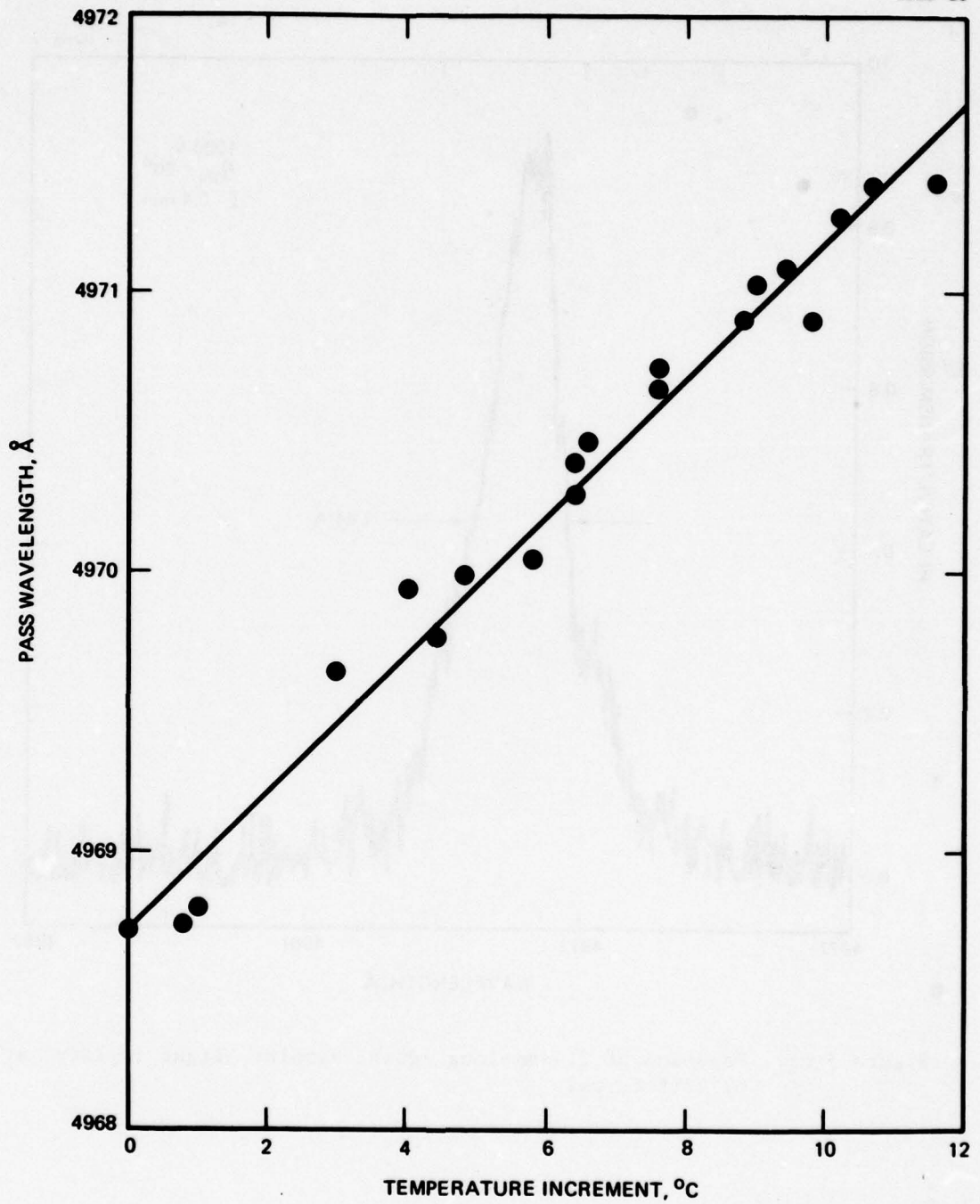
Figure 6. Variation of pass wavelength with temperature in \text{AgGaS}_2 iso-index filter.
