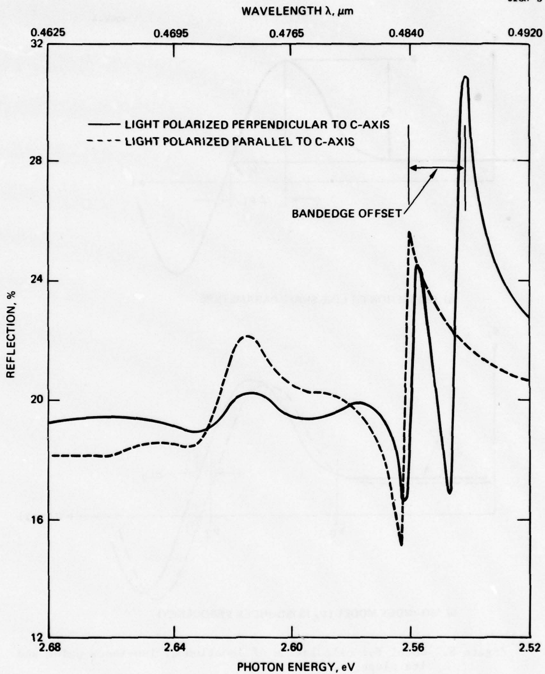
Figure 7. Reflection as a function of wavelength at 77°K for hexagonal, single-crystal cadmium sulfide. (Taken from Ref. 7.)
