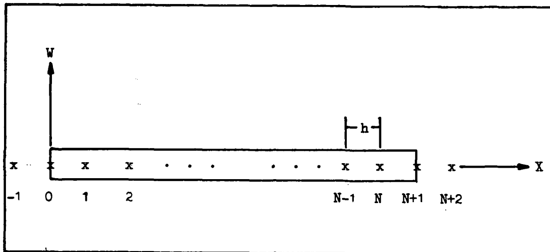
Fig 4. Node Pattern for N Internal Nodes
