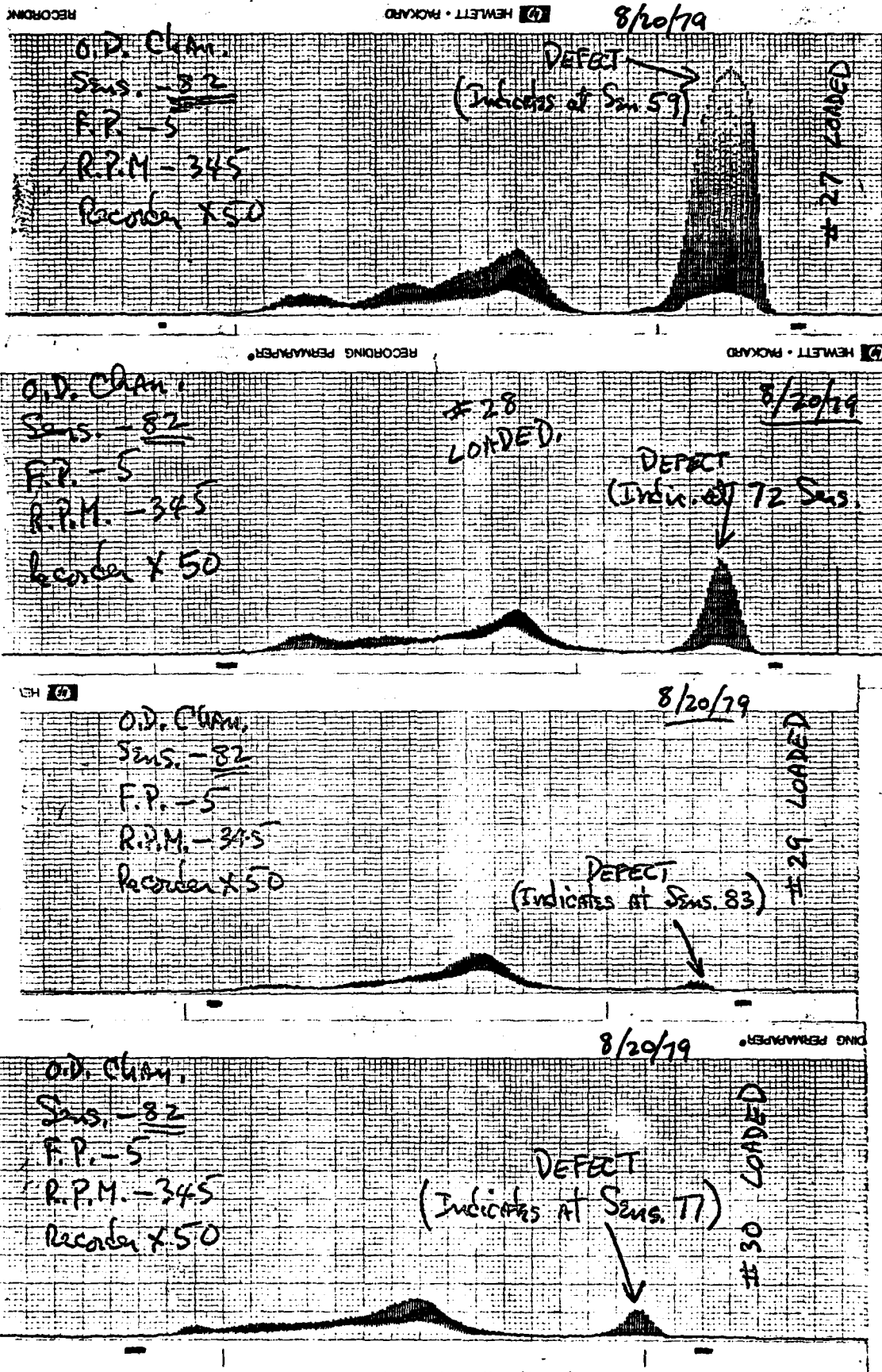
Transverse Magnetization
