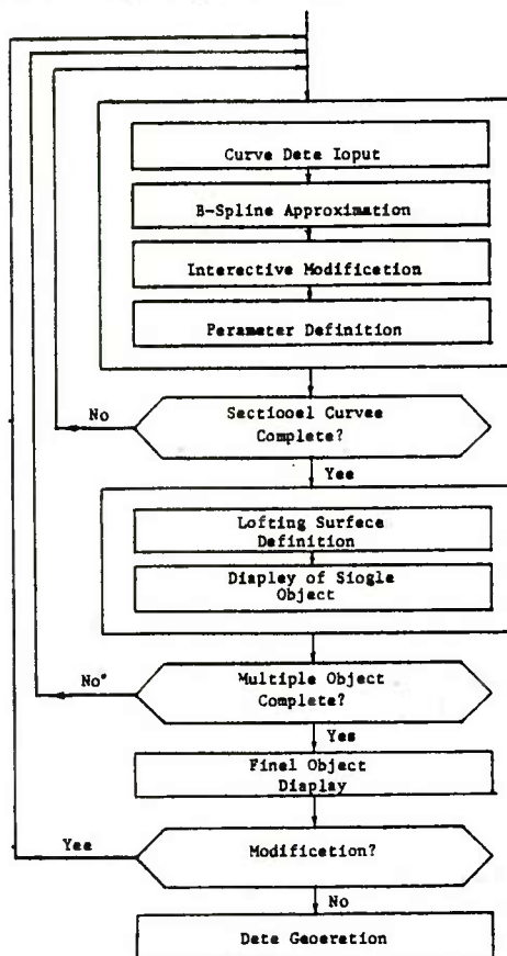
Fig. 6. Flowchart of program organization.
