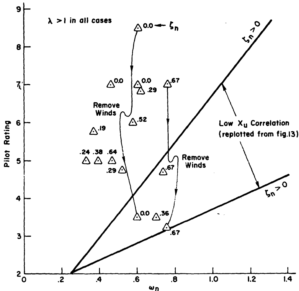
Figure 20. Pilot Rating vs. Frequency for Large X_u ( X_u = -0.2 )
