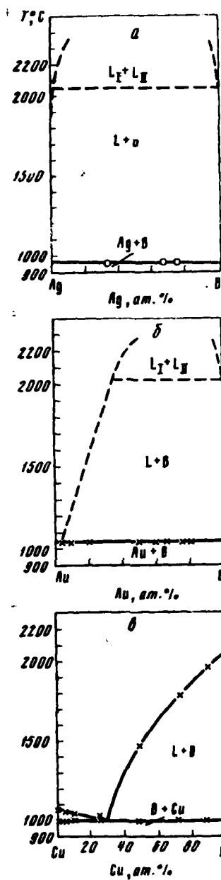
Fig. 5. Ag - B (a), Au - B (b) and Cu - B (c) systems /1/
