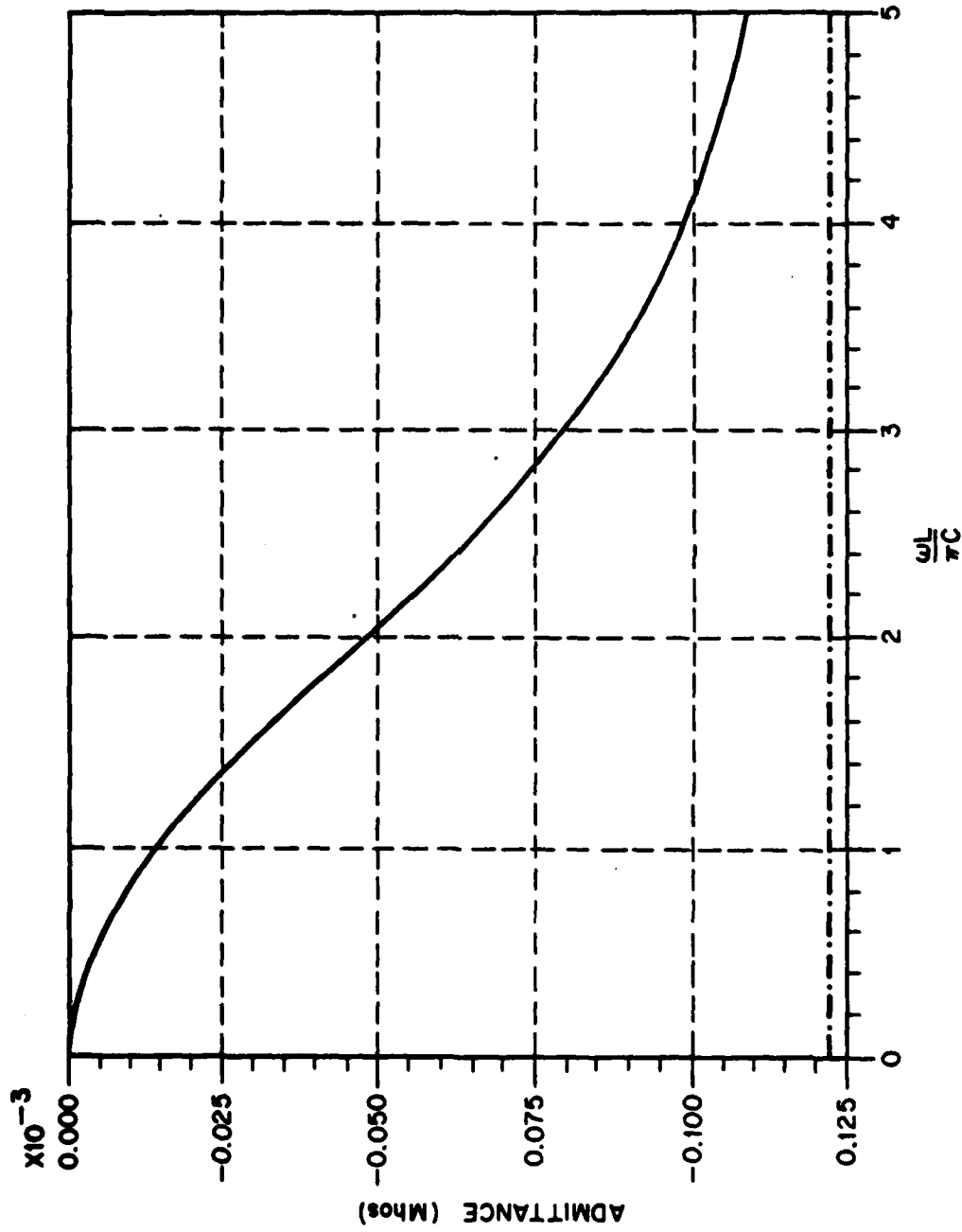
Figure 30: Real part of straight wire pole-pair admittance at z/L = .25 for pole 2, second layer.
