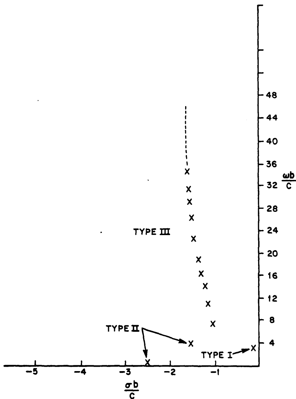
Figure 10: Classification of SEM poles for the circular loop into type I, type II, and type III.
