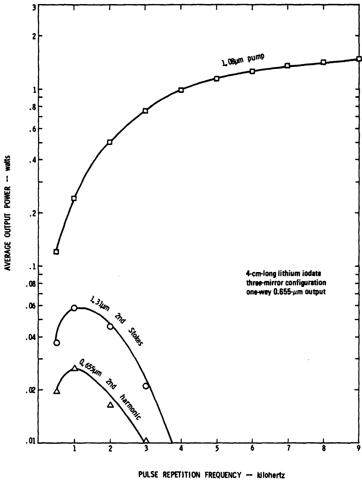
Figure 23. Pump, second-Stokes, and (one-way) 0.655 \mu m SH average powers
