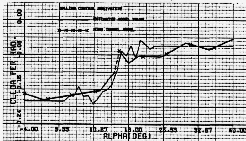
Figure 3.3-2 Comparison between the identified model and the T-2C wind tunnel data for C_{l\delta_a} .
