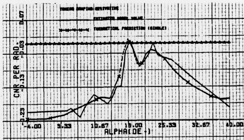
Figure 3.3-7 Comparison between the C_{n_r} identified model and the theoretical prediction model of Bihrl Applied Research
