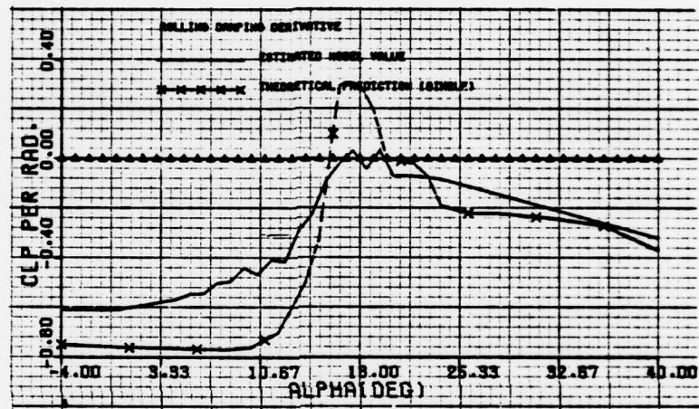
Figure 3.3-3 Comparison between the C_{l_p} identified model and the theoretical prediction model of Birle Applied Research
