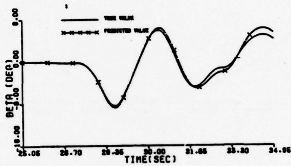
Figure 2.5-3 Comparison between the predicted and the true time histories of \alpha and \beta for the new maneuver
