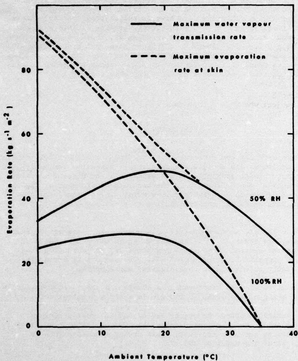
Figure 6. The maximum rate at which water vapour can escape from a Gore-tex rainsuit for varying ambient temperature. Also shown, for comparison, is the maximum rate at which sweat can evaporate from the skin. A significant fraction of the evaporated sweat can escape.
