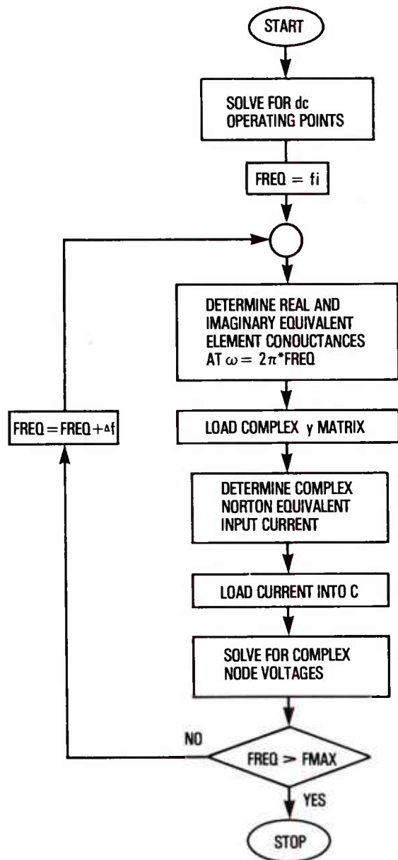
Figure 22. Flow diagram for traditional ac analysis procedure.
