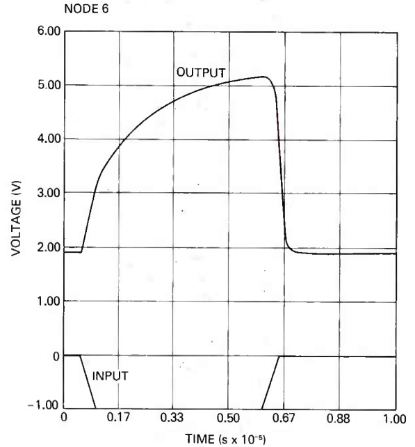
Figure 12. Input pulse and pulse response for CKT13 using BIAS-D.
