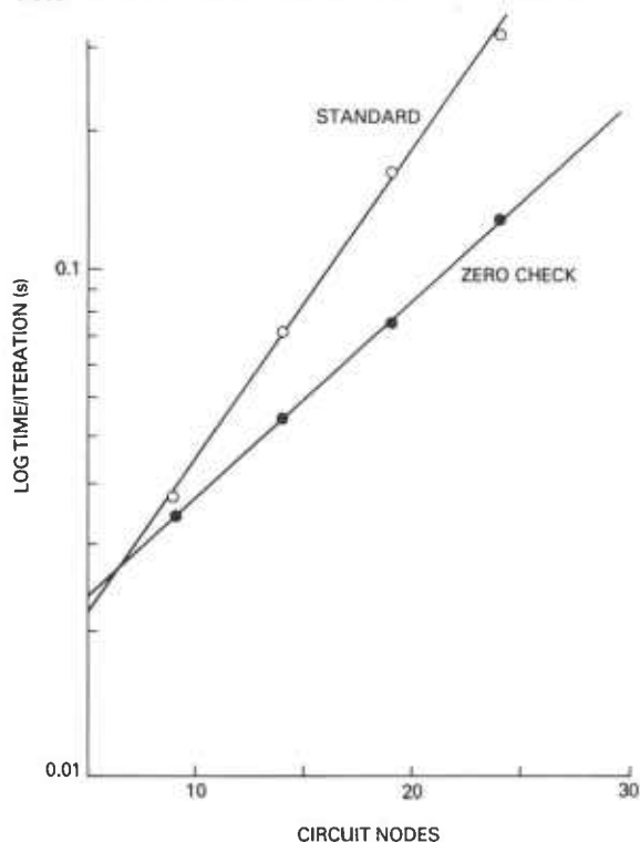
Figure 13. Speed versus circuit nodes for BIAS-D (PRIME 400) using zero test compared with standard version using test circuits.
