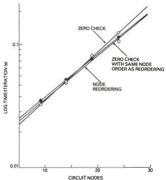
Figure 14. Speed versus circuit nodes for BIAS-D (PRIME 400) using node reordering.
