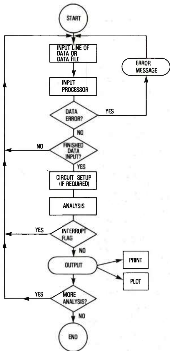
Figure 11. Flow diagram for an interactive circuit-simulator input processor.
