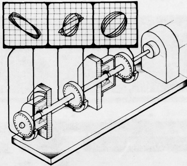
Figure 5. - Rotor bearing system used as example problem.
