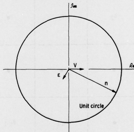
Figure 4. - Complex plane.
