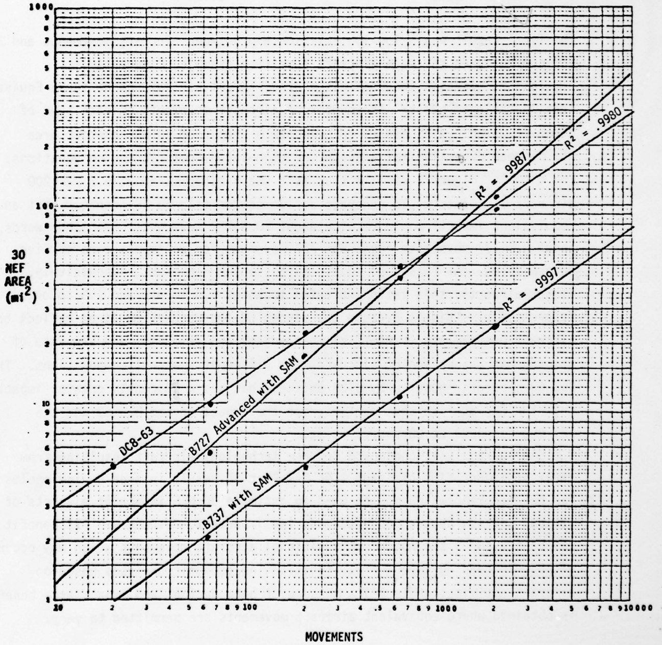
FIGURE 1. 30 NEF AREA VS. MOVEMENTS FOR 727, 737 AND DC8
