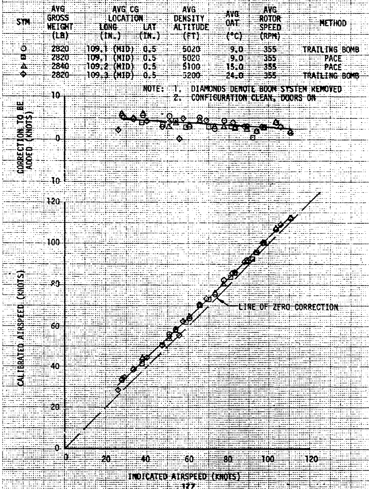
FIGURE 100 SHIPS SYSTEM AIRSPEED CALIBRATION IN LEVEL FLIGHT OH-58C USA S/N 68-16724
