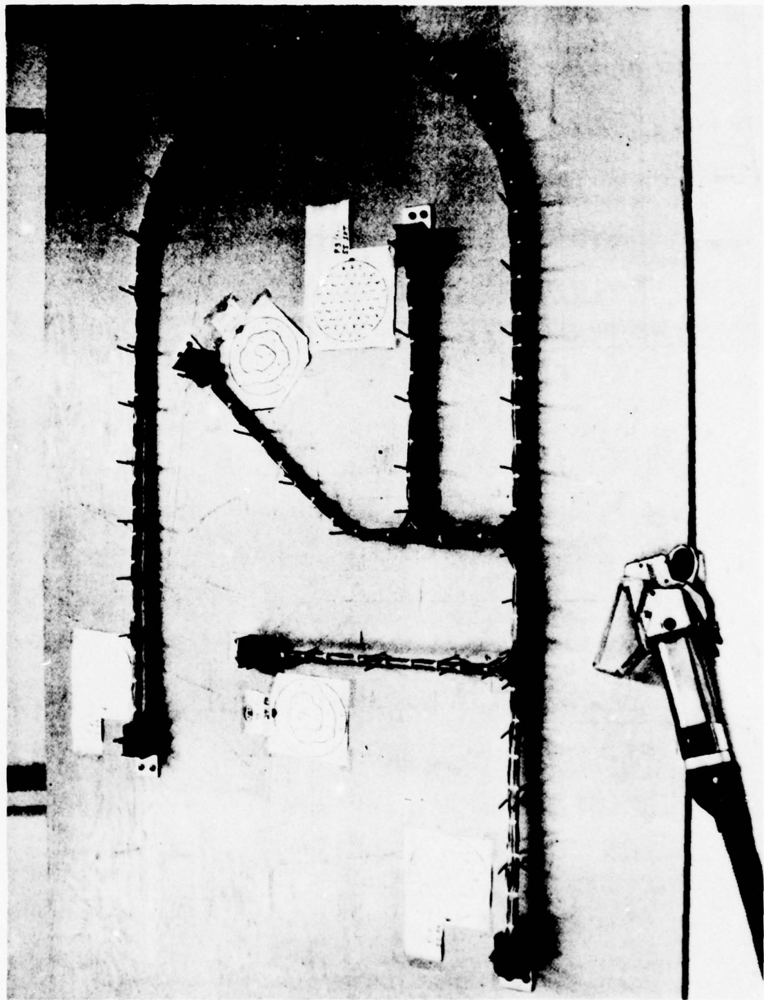
Figure A-3. A Representative Sample of a Missile Harness Assembly
