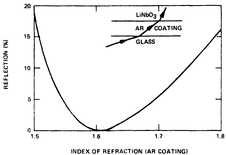
FIG. 7 Reflection vs. index of refraction of AR coating.
