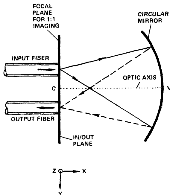
FIG. 11 Optical ray paths within terminal.
