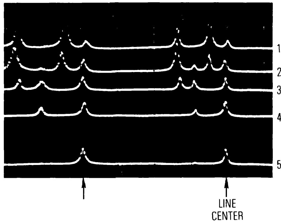
Fig. 7. Mode power spectra with competition and asymmetries of the modes in a stable resonator shown. R_1 = 3 \text{ m} , R_2 = \infty , and L = 200.5 \text{ cm} at various aperture openings. Traces 1 and 5 were obtained when the aperture was fully opened and fully closed (2 mm in diameter), respectively. Traces 2, 3, and 4 were obtained when the aperture was at intermediate aperture openings. Arrows indicate line center. Vertical scale is 0.2 V/div and horizontal scale 18 MHz/div
