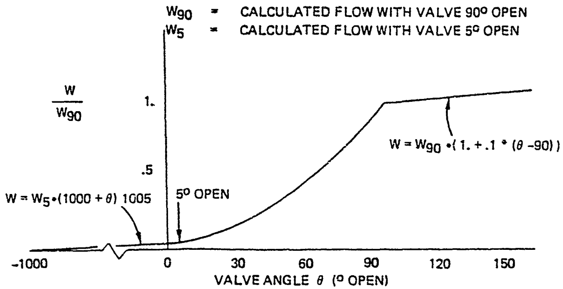
Figure 2 (a) Flow Calculation for Butterfly Valves
