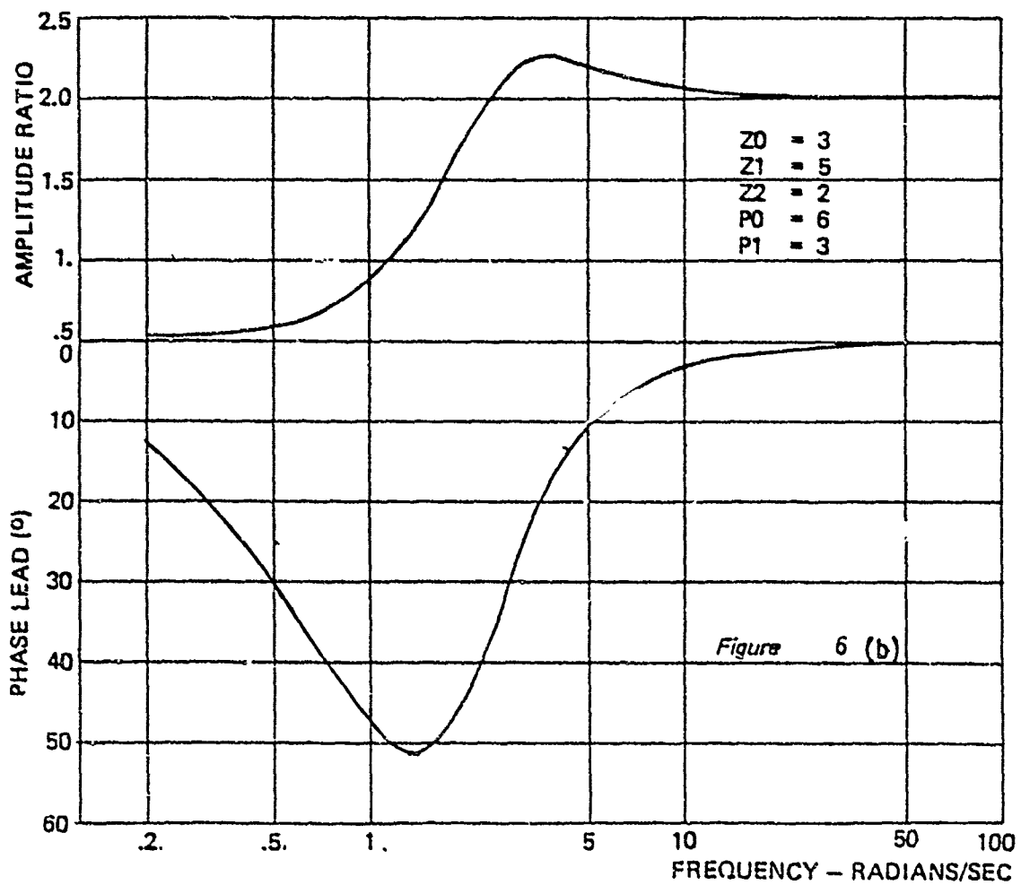
Figure 6 Typical Response for Subroutine TZ
