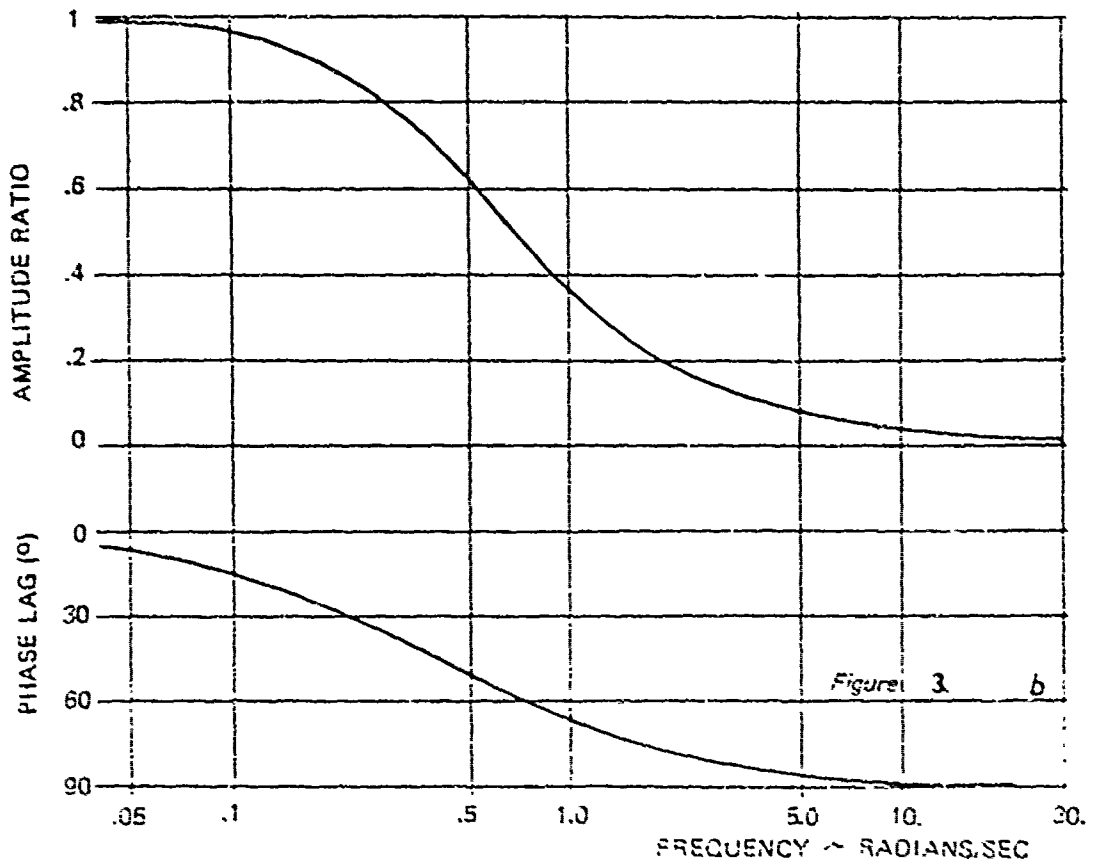
Figure 3 Typical Response for Subroutine LA
