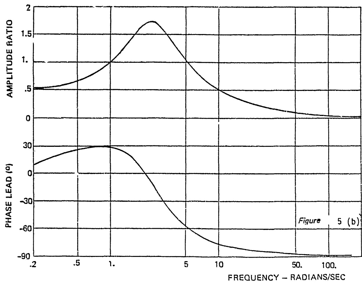
Figure 5 Typical Response for Subroutine TF
