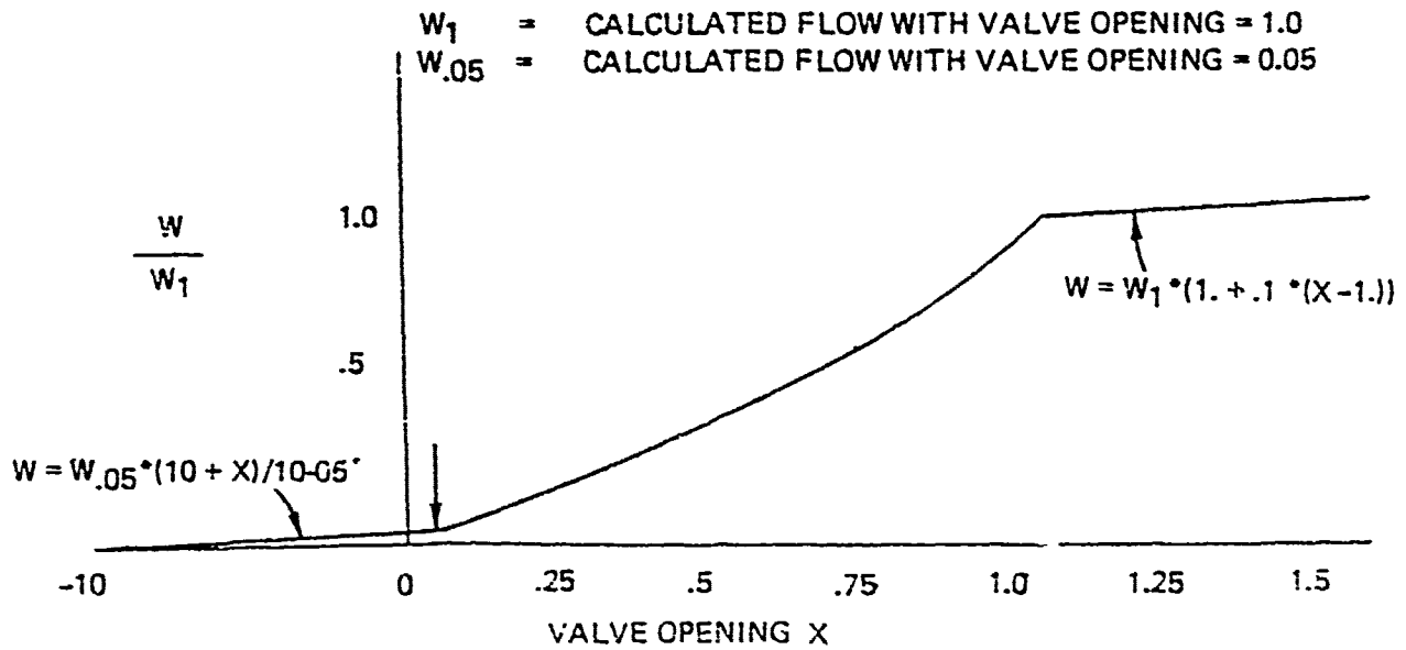
Figure 2 - (b) Flow Calculation for Globe and Gate Valves
