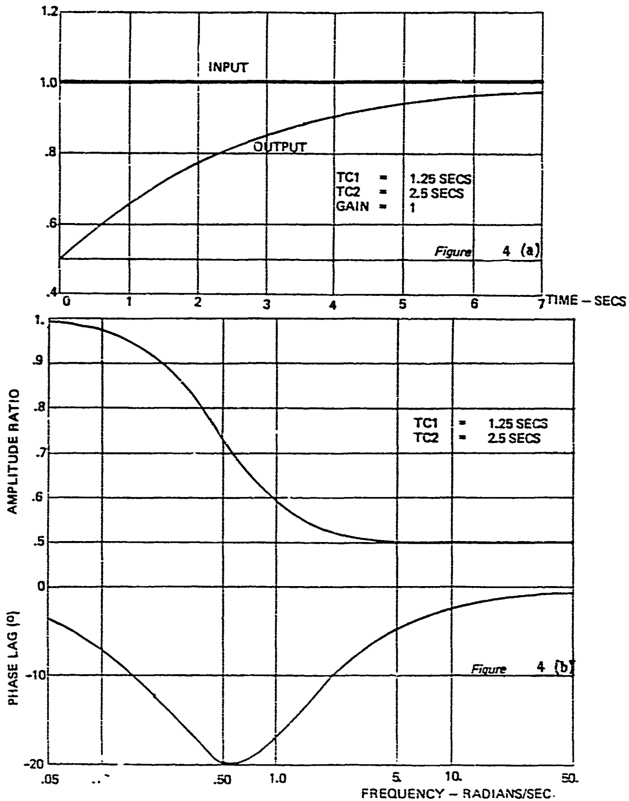
Figure 4 Typical Response for Subroutine LL
