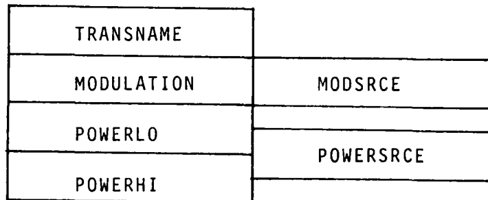
Figure 28. Transmitter Record
