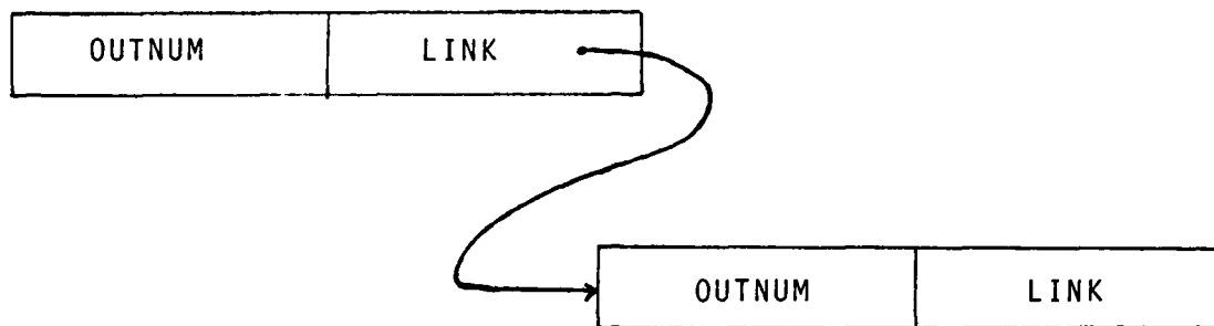
Figure 36. Output Type Record
