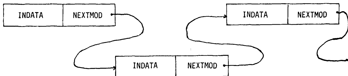
Figure 38. Modification Record
