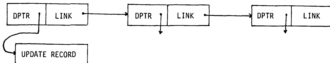
Figure 39. Chain Record
