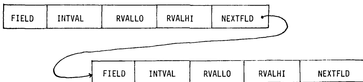
Figure 41. Query Record
