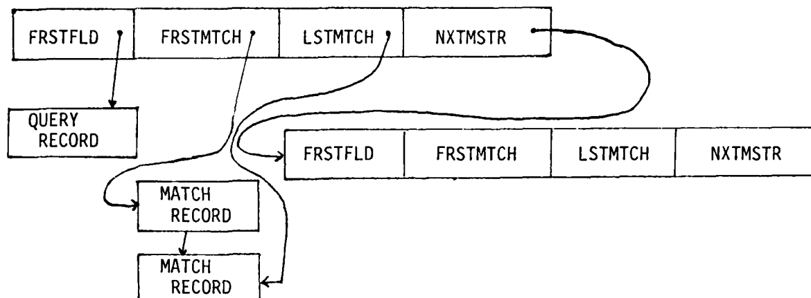
Figure 40. Query Master Record
