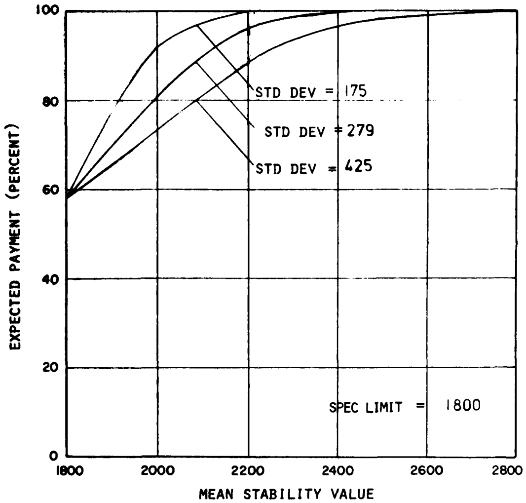
FIGURE 4.7 EXPECTED PAYMENT CURVE FOR THE PROPOSED STABILITY ACCEPTANCE PLAN FOR A STANDARD DEVIATION OF 175, 279 AND 425
