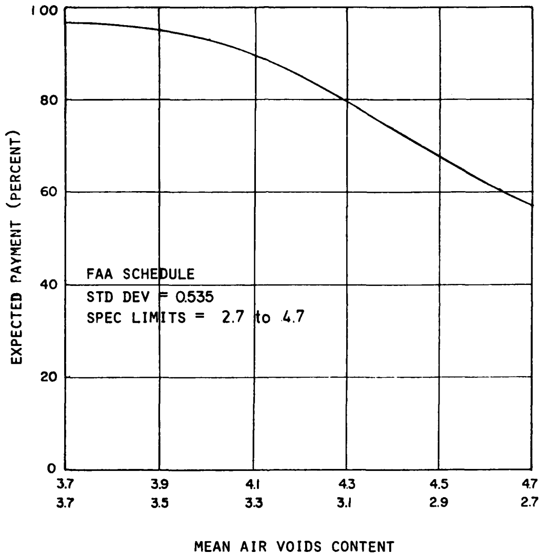
FIGURE 4.18 EXPECTED PAYMENT CURVE FOR AIR VOIDS CONTENT USING FAA PRICE ADJUSTMENT SCHEDULE FOR A STANDARD DEVIATION OF 0.535
