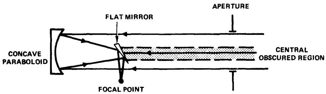
Figure II-3-a Newtonian Telescope
