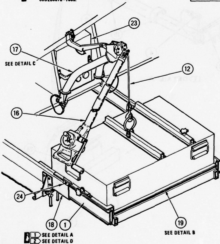
Figure 5-7. Transmitter (011) Installation and Removal Special Tools (Sheet 1 of 4)
