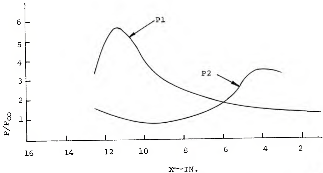
FIGURE 6 - SABOT UNDERSIDE PRESSURE PULSE GEOMETRY
