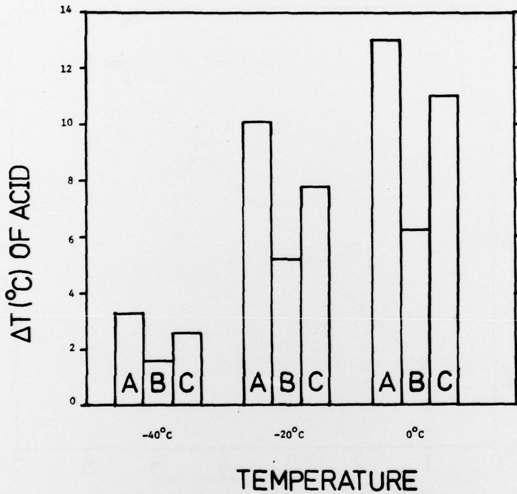
Fig. 11. The increase in acid temperature resulting from a 210A discharge
