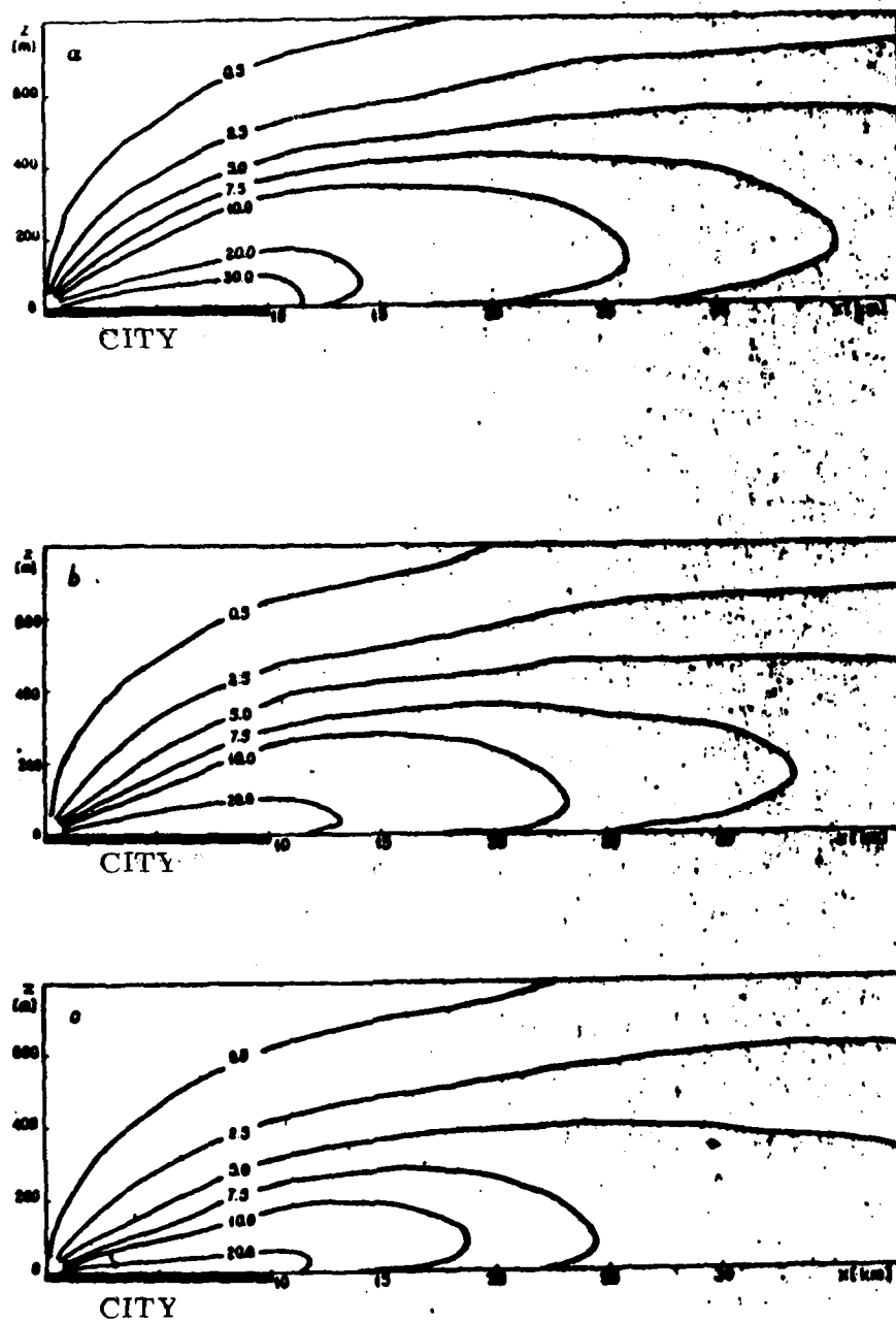
Fig. 3. Isolines of SO 2 concentration [ \mu\text{g}/\text{m}^3 ] a - G = 3 \text{ m/s} ; b - G = 6 \text{ m/s} ; c - G = 10 \text{ m/s}
