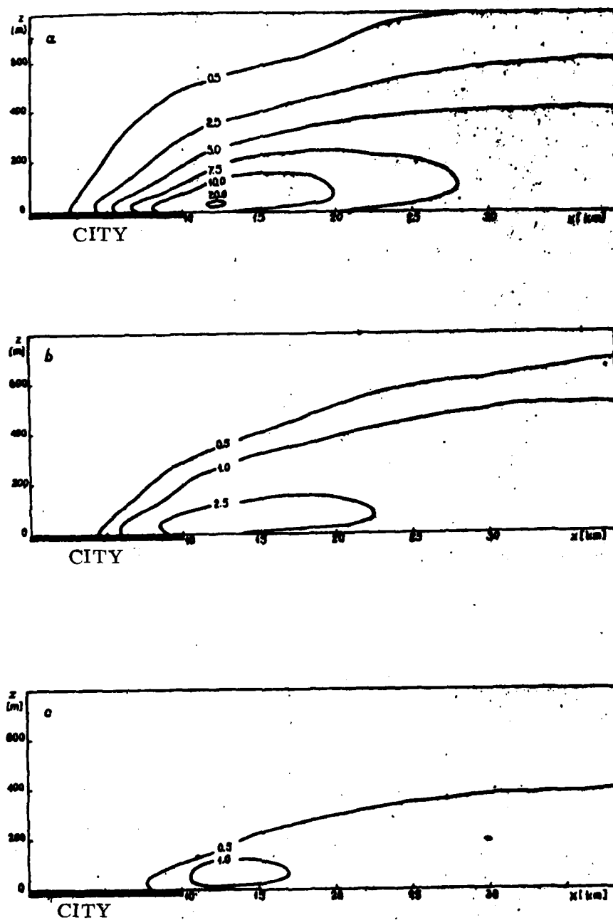
Fig. 4 Isolines of \text{H}_2\text{SO}_4 concentrations [\mu\text{g}/\text{m}^3] a - G = 3 \text{ m/s} ; b - G = 6 \text{ m/s} ; c - G = 10 \text{ m/s}
